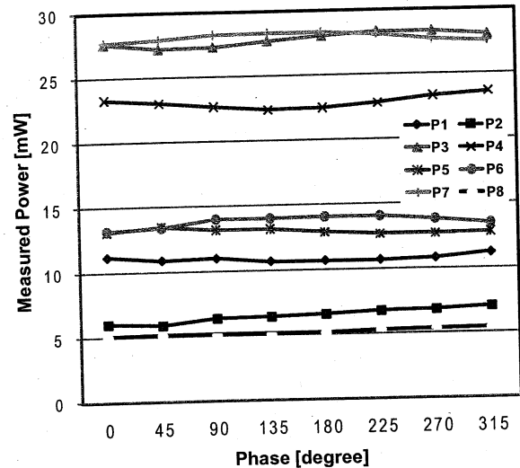
Fig. 7. Measured power versus phase.
