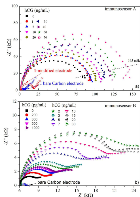
Figure 4: Impedance spectra of the electrodes of immunosensors A and B exposed to difference concentrations of \alpha -hCG. The impedance results were obtained in the solution containing 0.1M KCl and 5mM K_3[Fe(CN)_6]/K_4[Fe(CN)_6] at OCP and frequency range is from 100 kHz to 50 mHz with an Ac probe amplitude of 10mV.
