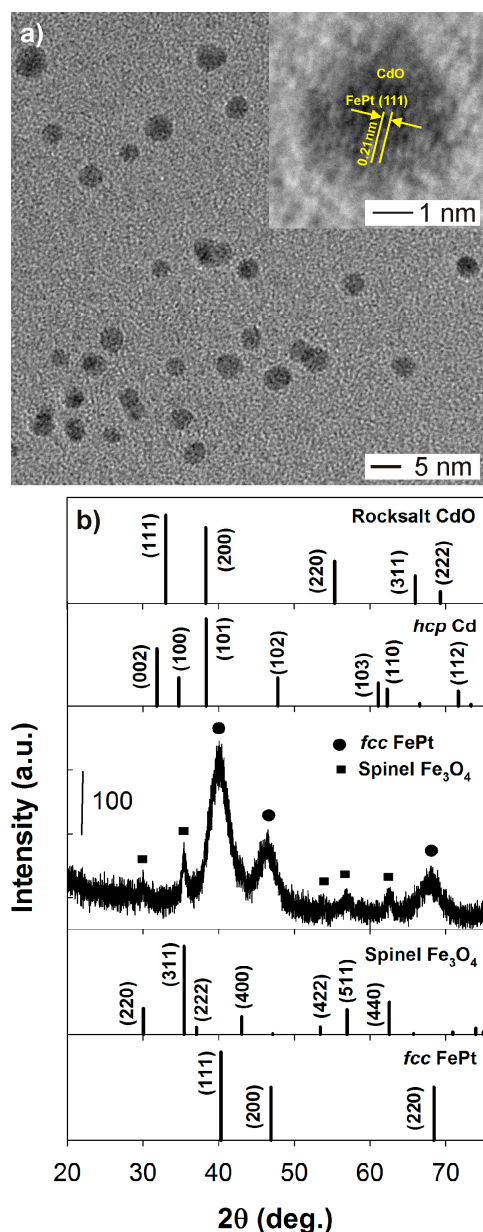
Fig. 2. (a) TEM image of intermediate NPs (B). The inset shows a HRTEM image of a single NP. (b) XRD pattern of intermediate NPs with reference peaks for fcc FePt (JCPDS card no. 00-029-0718), Fe 3 O 4 (01-079-0419), Cd (00-005-0674) and CdO (003-065-2908). Composition measured by EDS is Fe:Pt:Cd = 37:38:25.
