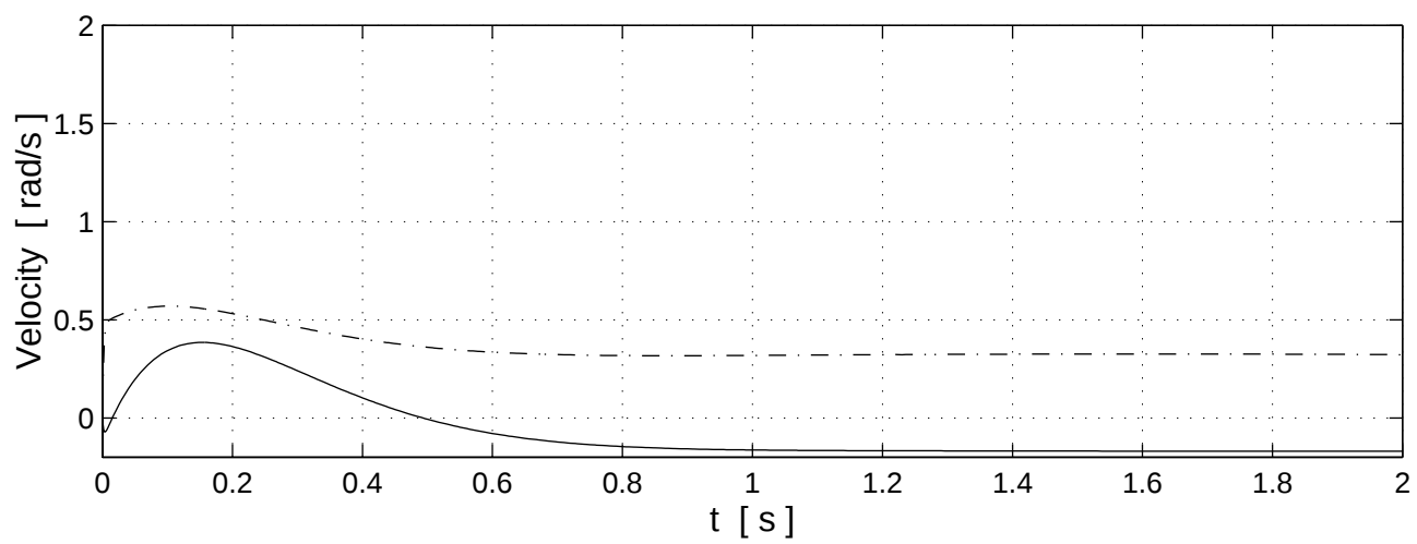
Figure 5.7: Image Error and Velocity
