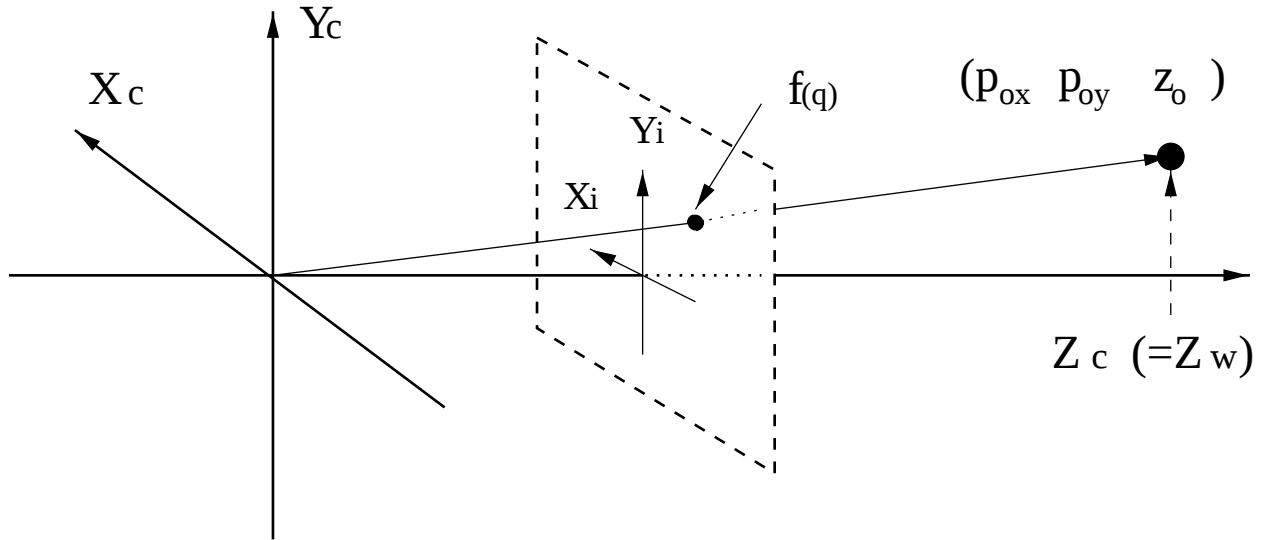
図 2.2: The coordinate frame for the camera system
