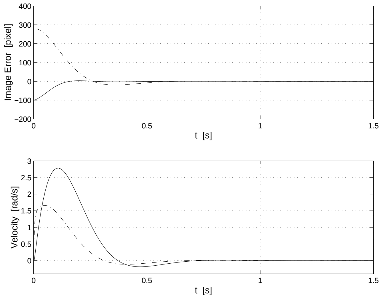
⊠ 4.2: Image Error and Velocity ( k_p = 0.20 , k_v = 5.0 )
