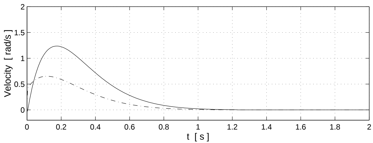
Figure 5.1: Image Error and Velocity
