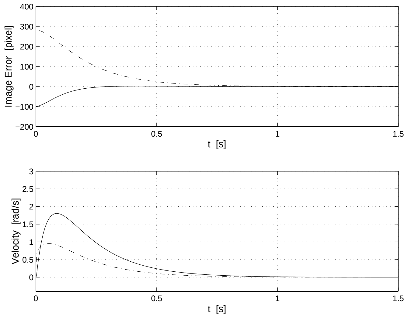
Fig 4.3: Image Error and Velocity ( k_p = 0.20 , k_v = 10 )
