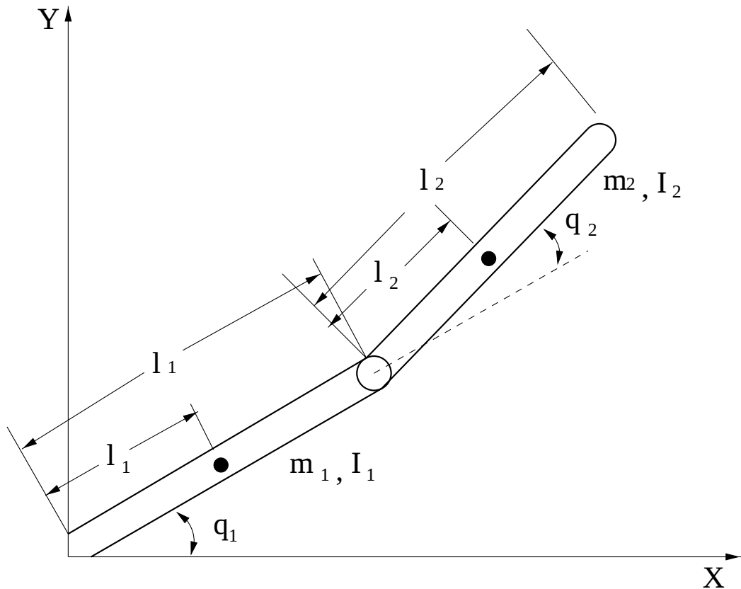
図 4.1: Two-link planar robot
