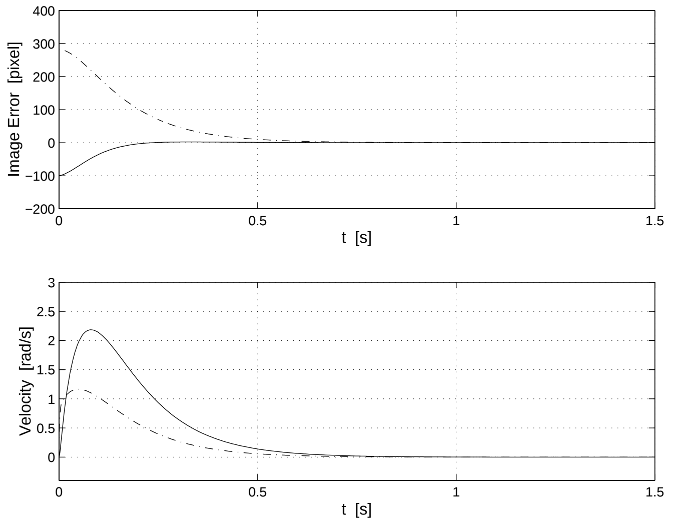
Fig 4.4: Image Error and Velocity ( k_p = 0.25 , k_v = 10 )
