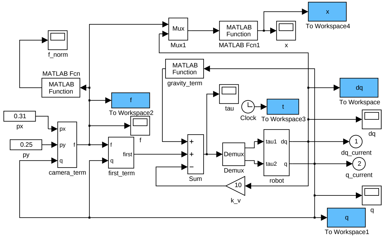
6.1: Block diagram of visual servo system
