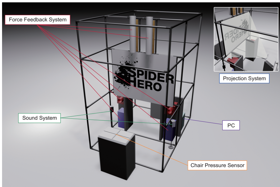
Figure 4: System layout.
