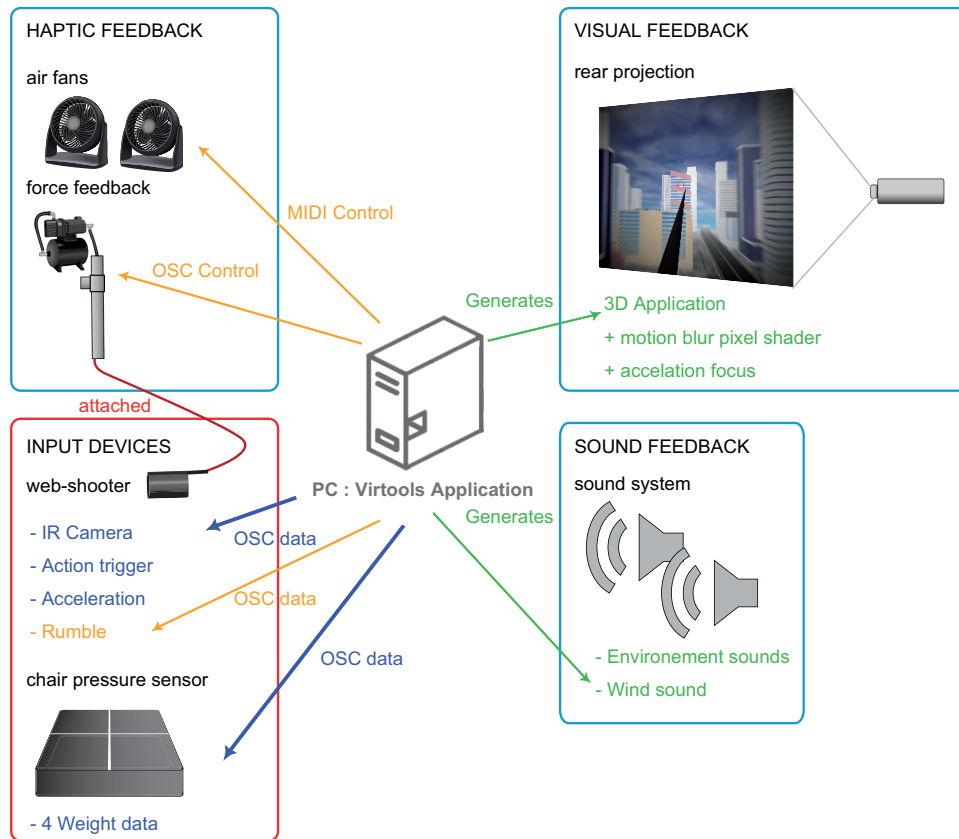
Figure 3: System overview.
