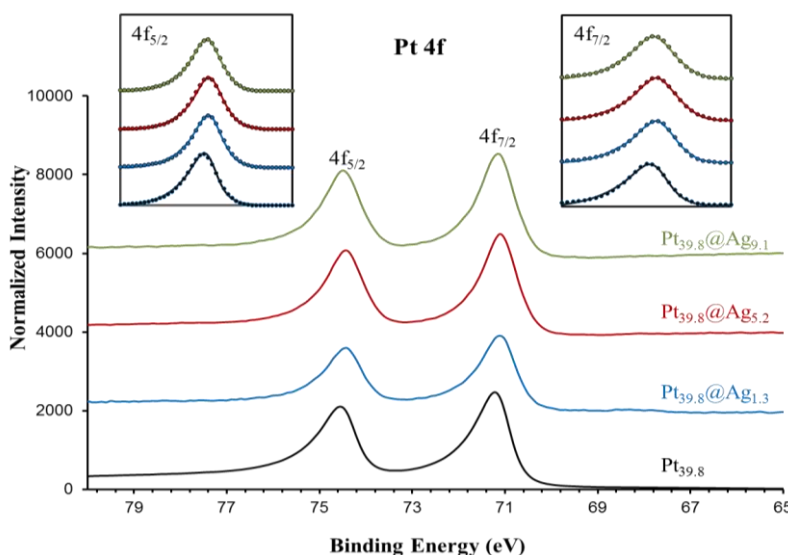
Figure 8. XPS spectra for platinum core particle (39.8 nm) (A) and Pt 39.8 @Ag y particles with an optimal silver shell thickness of 1.3 (B); 5.2 (C); and 9.1 (D) nm. The inserted graphs show the Pt 4f 7/2 and 4f 5/2 peaks (solid curves) and the fitting with the asymmetric G-L mixed function (circles).
