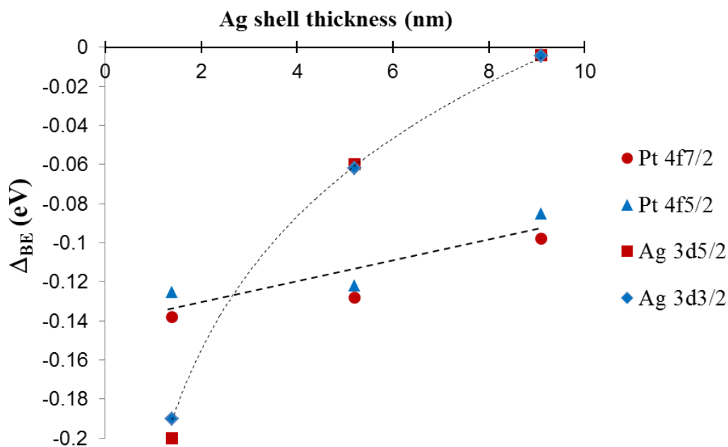
Figure 9. The Pt 4f and Ag 3d peak energy shift plotted as a function of silver shell thickness for Pt 39.8 @Ag y ( y = 1.3, 5.2, \text{ and } 9.1 \text{ nm} ) NPs. The peak energy shift \Delta_{BE} = BE_{\text{core-shell}} - BE_{\text{Pt}} (or BE_{\text{Ag}} ).
