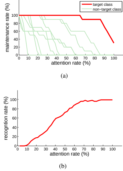
Fig. 2. Face recognition according to the attention rate. (a) maintenance rate for a target and non-target classes, (b) average recognition rate with 10 classes.
