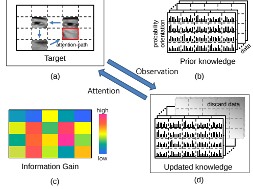
Fig. 1. Framework of attention path planning algorithm
