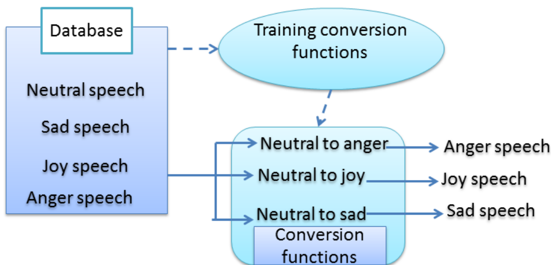
Figure 1.1: GMM method
