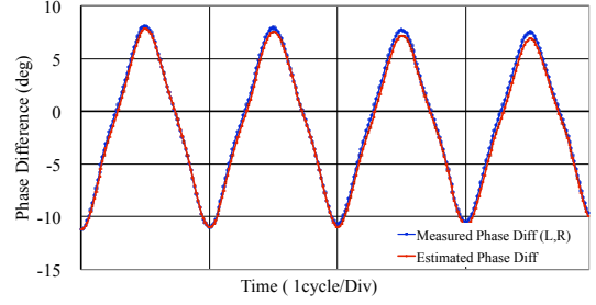
Fig. 11. Phase Angle Measurement
