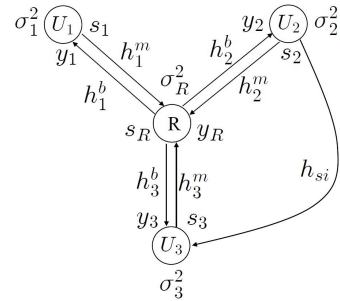
Fig. 1. Structure of three-way relay with side information from user U_2 .
