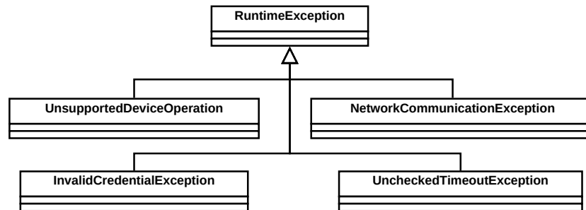
Figure 3.10: Defined Runtime Exceptions
