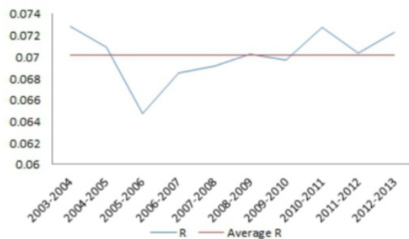
Fig. 2: Soccer's GR values for the years 2003-2013
