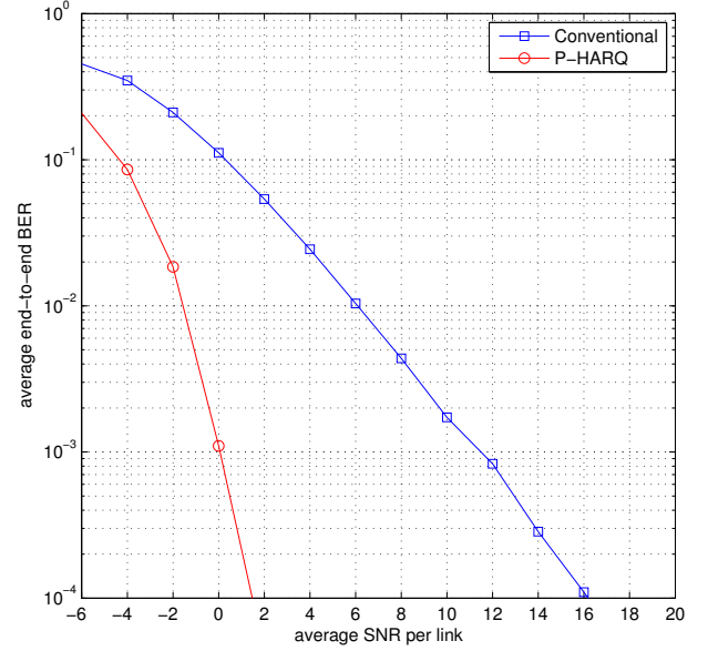
Fig. 4. BER performances.
