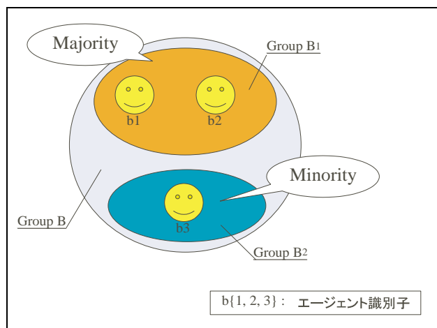
図 6.1: Majority Voting
