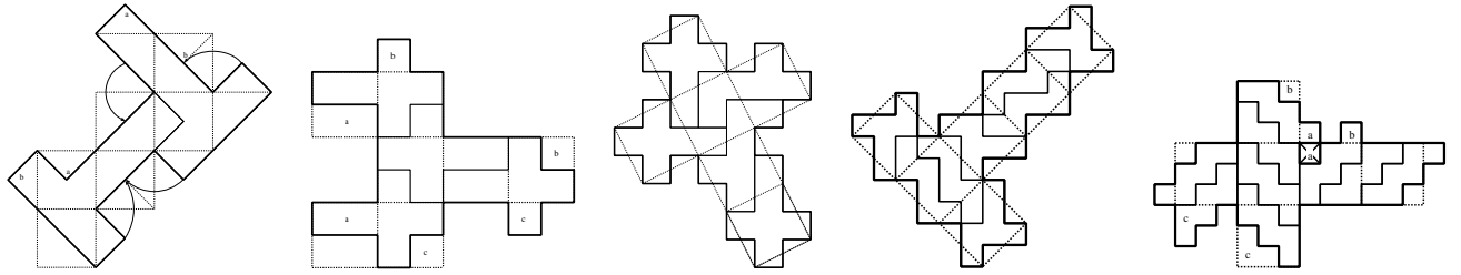
Figure 1: Rep-cubes of order k = 2, 4, 5, 8, 9 , respectively.
