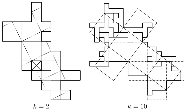
Figure 3: Patterns for non-regular rep-cubes of order k = 2, 10 .
