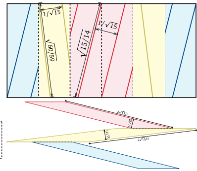
Figure 2: Patterns for rep-cubes of order k = 36, k = 64 , and k = 50
