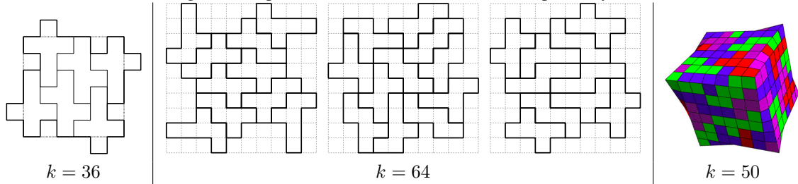
Figure 2: Patterns for rep-cubes of order k = 36, k = 64 , and k = 50
