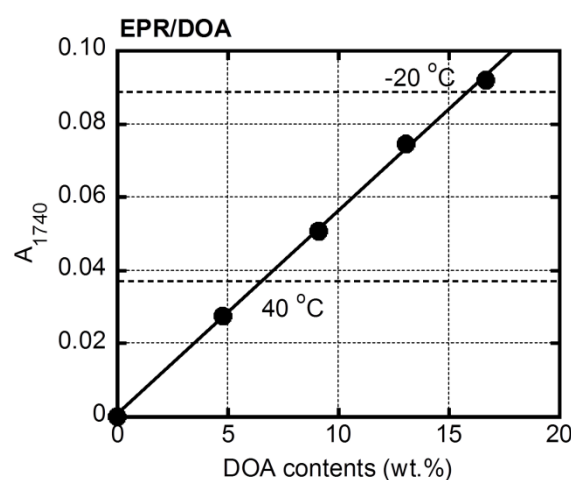
Fig. 5 Absorbances at 1740\text{ cm}^{-1} for the EPR/DOA sheets containing various amounts of DOA. The absorbances after annealing are also indicated by the dotted lines.
