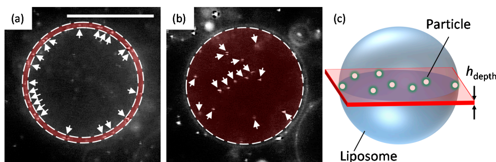
Figure 7. Regions for counting (a) fully wrapped particles and (b) penetrated particles. The white arrows indicate particles. Scale bar is 20 \mu\text{m} . (c) Schematic of the region observed by an optical microscope.
