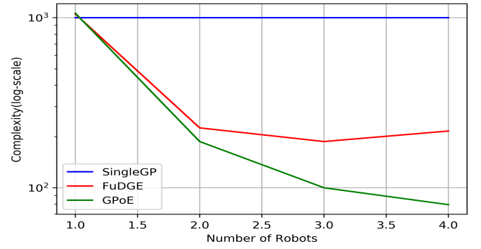
(b) Complexity v/s Number of Robots
