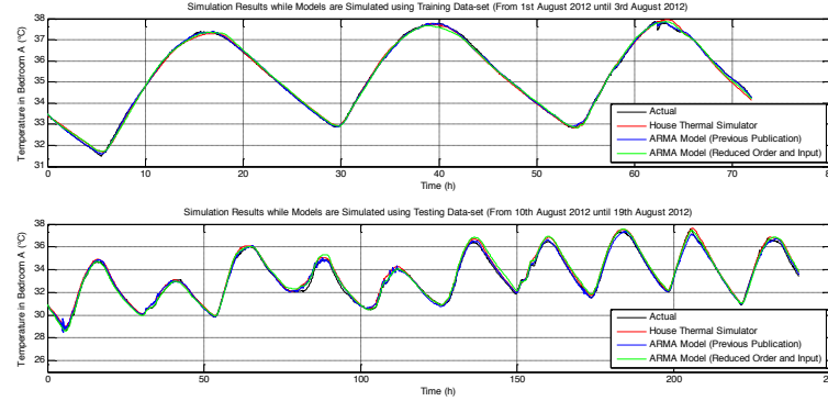
Fig. 4. The simulation result comparison for all three optimized models when simulated with training data set and testing data set.
