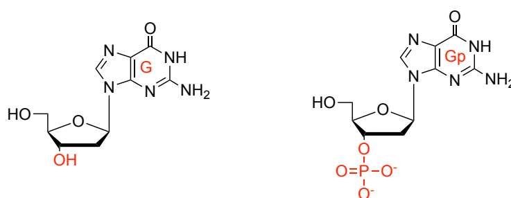
Figure 5.2: Structure of modified counter base.
