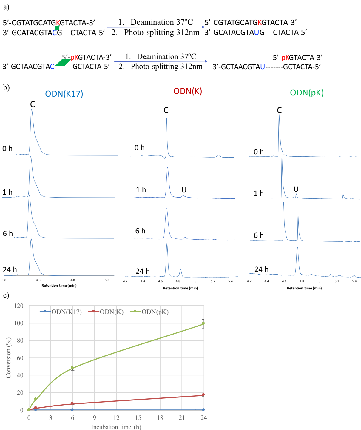
Figure 5.8: a) Scheme of deamination. b) UPLC chromatograms for deamination of ODN(tC) using ODN(K) and ODN(pK). Sample: photo-cross-linked duplexes (2.5 \mu\text{M} ) in 50 mM sodium cacodylate buffer containing 100 mM NaCl were incubated at 37°C (photo-splitting: 312 nm, 121.3 mW/cm 2 , 37°C). c) Time course of deamination reaction.
