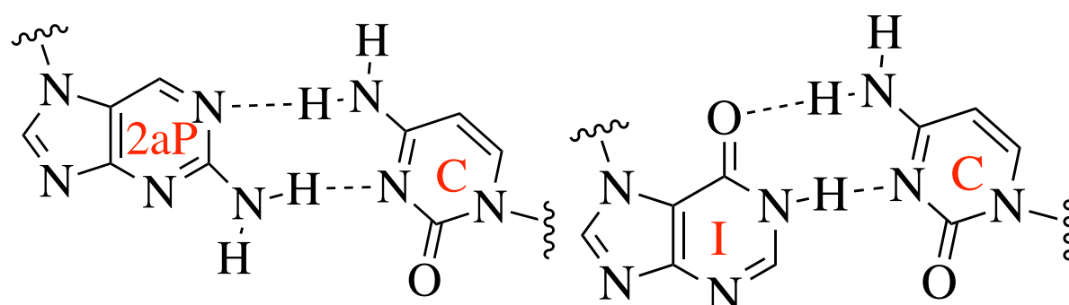
Figure 2.9: Hydrogen bonding comparison in 2-aminopurine and inosine
