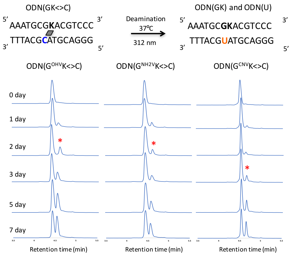
Figure 4.4. UPLC analysis of the deamination reaction of the photo-cross-linked duplex consisting of ODN(GK) and cODN(C). [ODN(GK<>C)] = 5 μM in 50 mM Na-cacodylate buffer (pH 7.4) containing 100 mM NaCl. incubated at 37°C, photo splitting was performed with transilluminator (312 nm) at 37°C. Peak marked with asterisk indicate the newly formed ODN(U).
