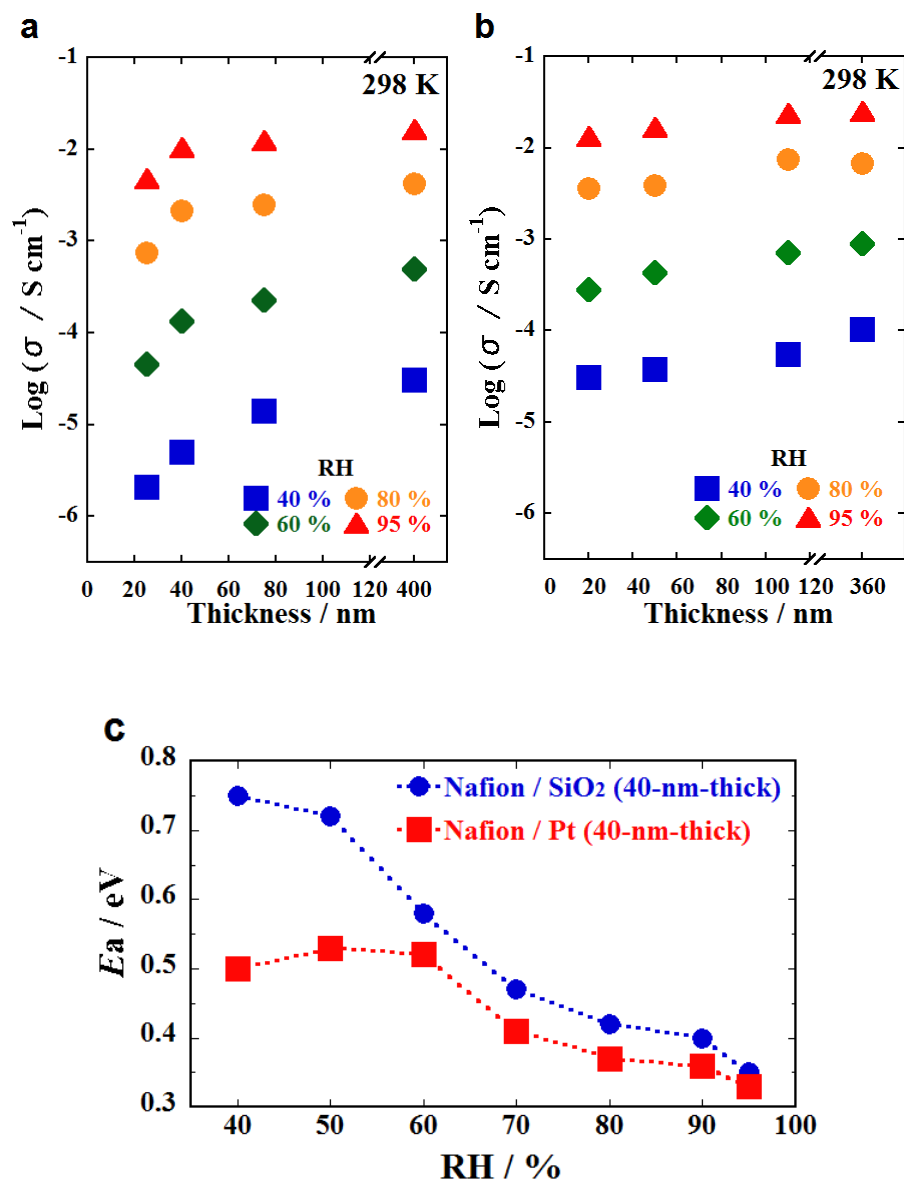
Figure 2. (a), (b) Thickness dependence of proton conductivity for Nafion thin films at various relative humidity (RH): (a) on SiO 2 and (b) on Pt-deposited surface. (c) Activation energy for the 40-nm-thick Nafion thin films on SiO 2 and Pt-deposited surface as a function of the RH. Adapted with permission from ref 65. Copyright 2016 American Chemical Society.
