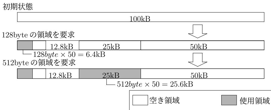
図 3.3: Block buddy system
