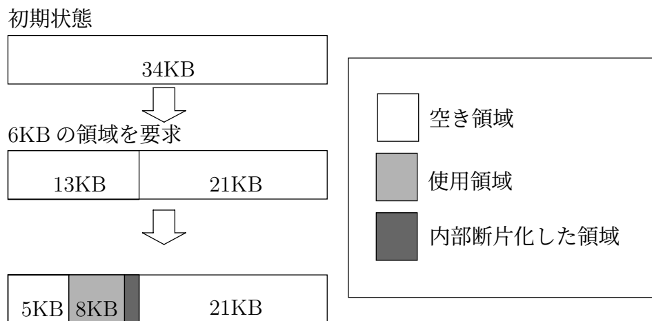
図 2.4: Fibonacci buddy system
