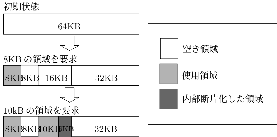
図 2.3: Binary buddy system
