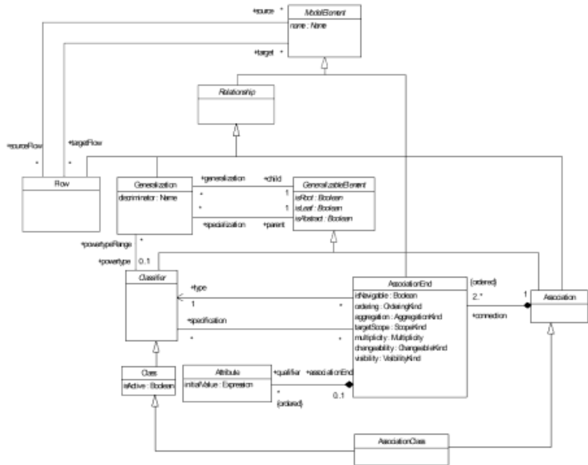
图 2.15: Core Package - Relationships
