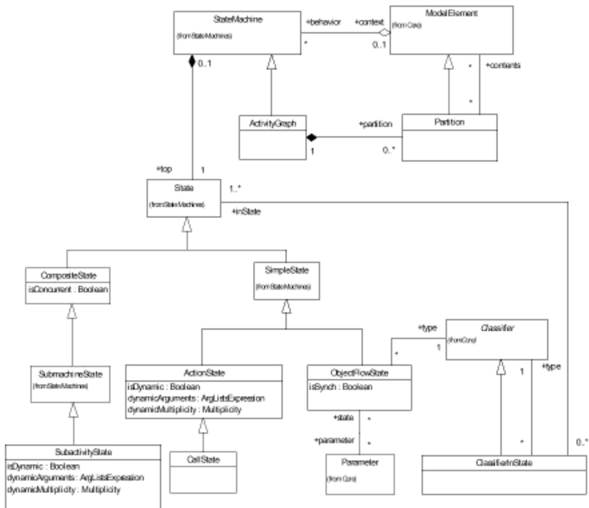
图 A.14: Activity Graphs
