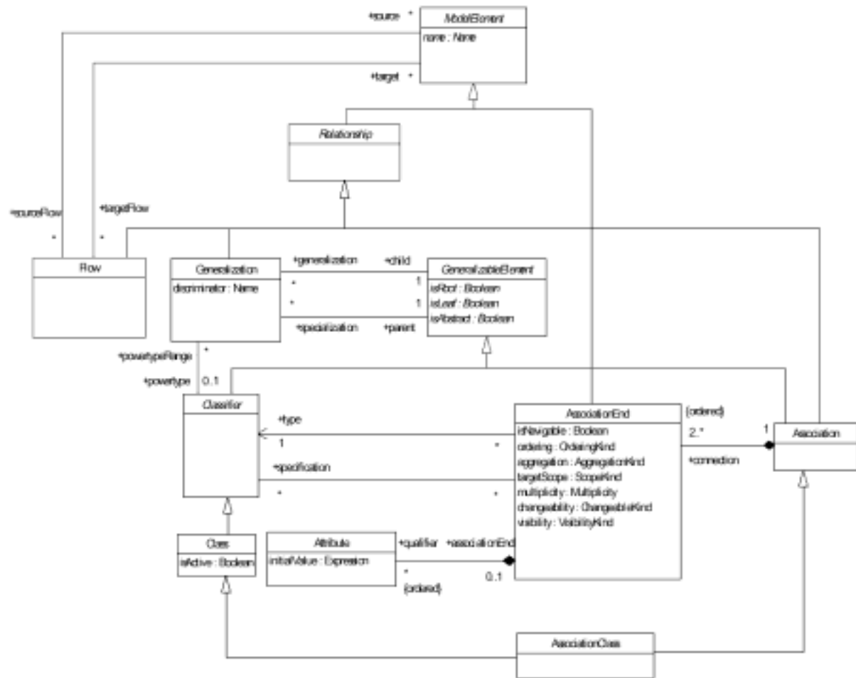
图 A.2: Core Package - Relationships
