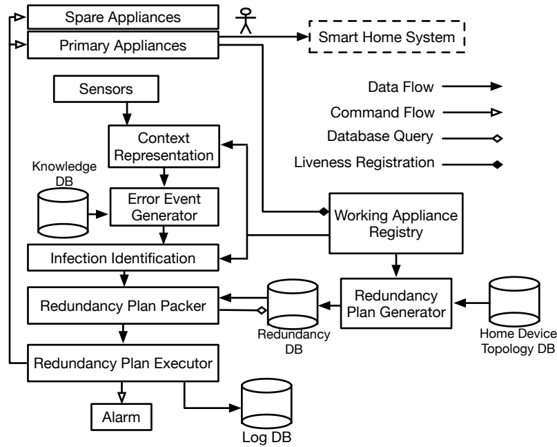
Figure 4.11: The components of the proposed redundancy model.
