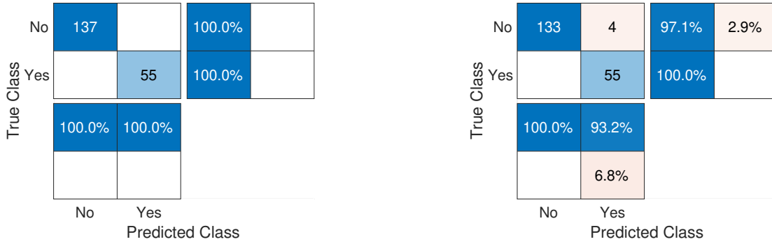
Figure 5.9: Example output of faked data.
