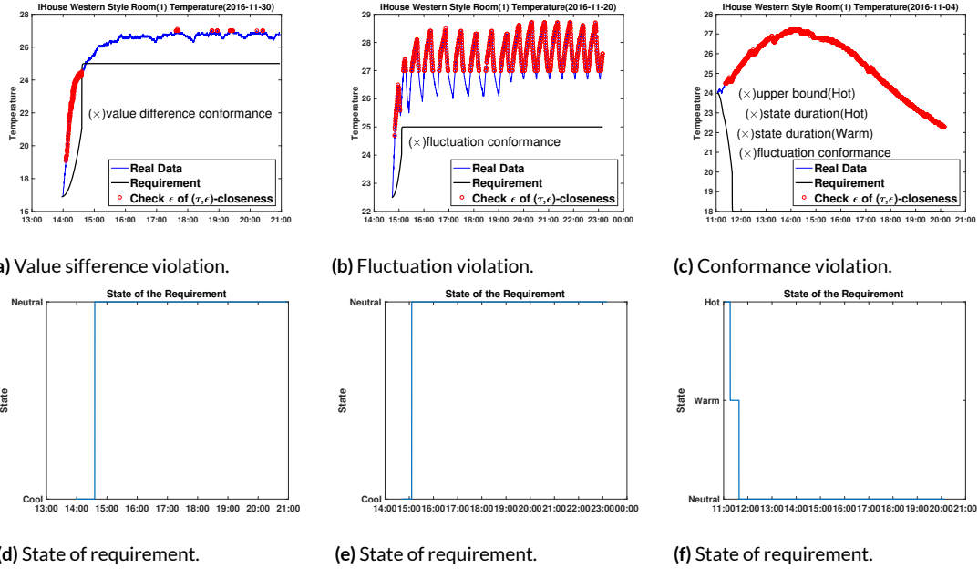
Figure 5.6: Results of the conformance check.
