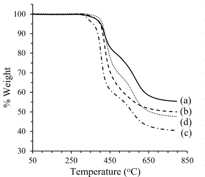
Figure 4.6 TG curves recorded under N 2 of PIs particles prepared from DKP-4APhe with various dianhydrides (a) BTDA, (b) CBDA, (c) DSDA, and (d) PMDA.
