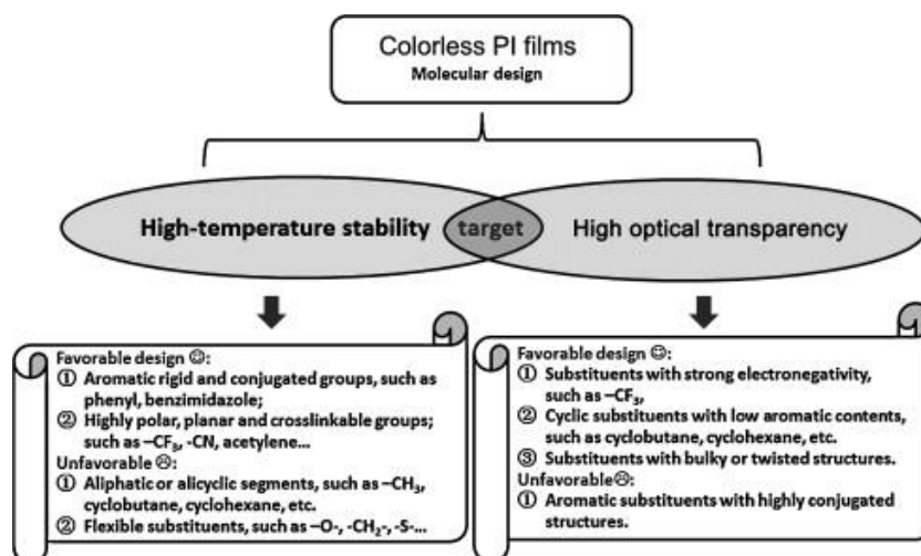
Figure 1.2 Molecular design for PI films [49].
