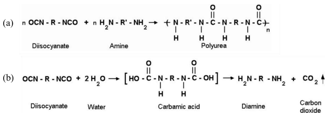
Scheme 1.3 (a) Polyurea chemistry and (b) Isocyanate/water reaction [73].
