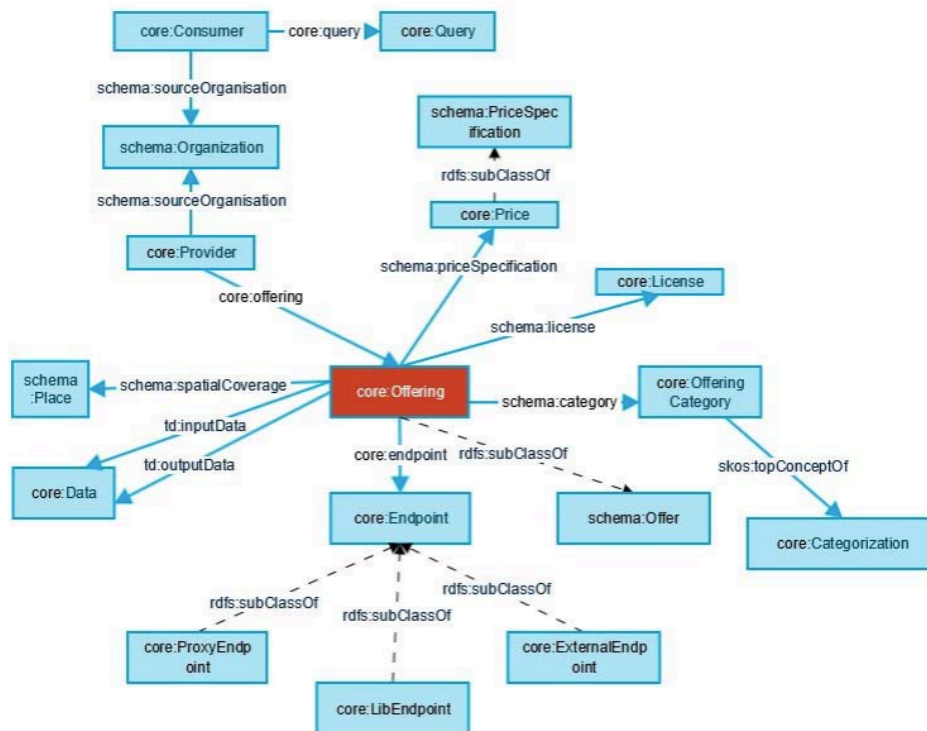
図 2.25 BIG IoT semantic core model
