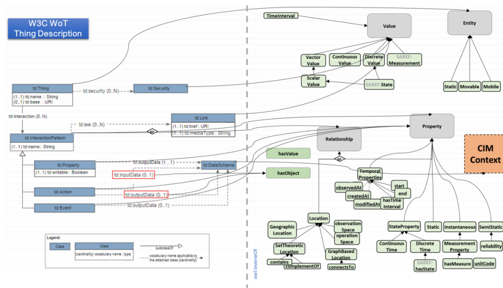
2.18 NGSI Mapping to WoT-TD[17]
