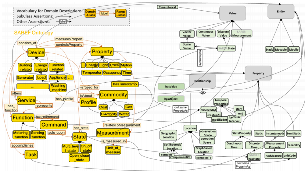
2.17 NGSI Mapping to SAREF[17]
