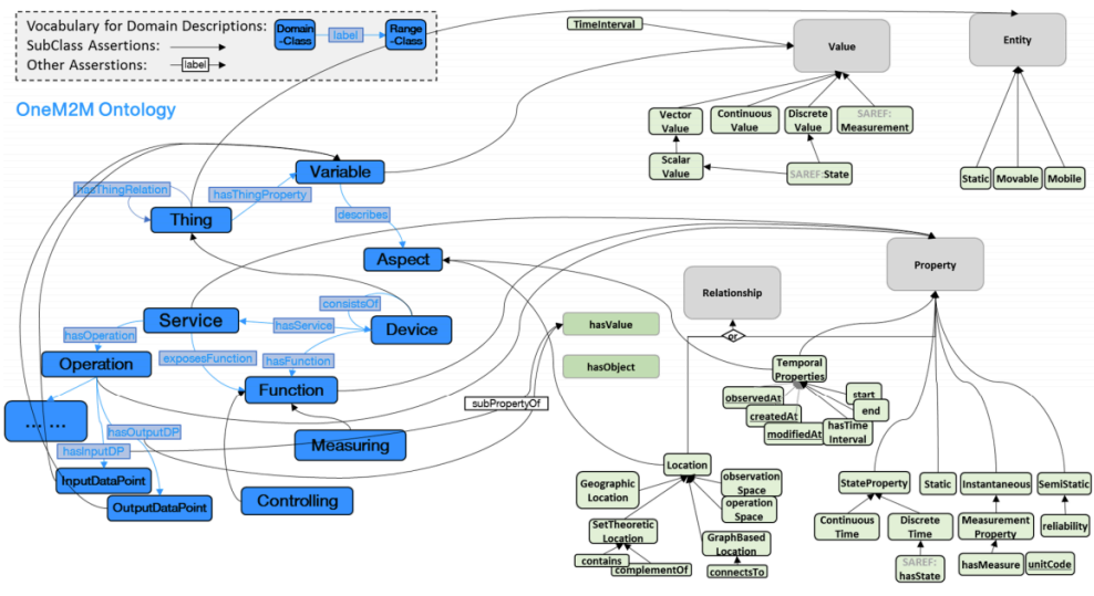
図 2.16 NGSI Mapping to oneM2M[17]
