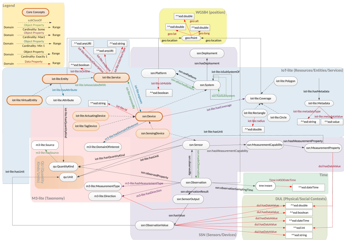
Figure 1: FIESTA-IoT Ontology
