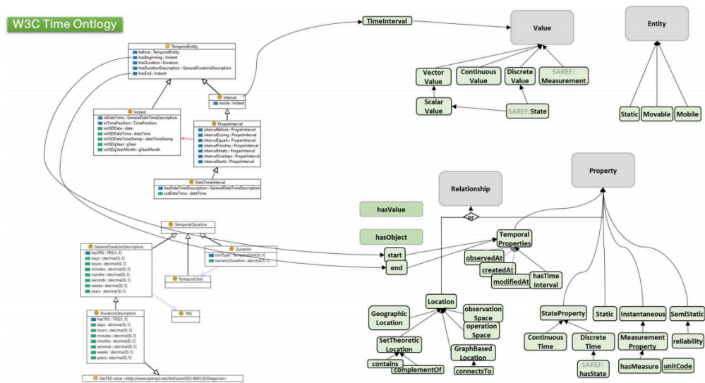
図 2.19 NGSI Mapping to W3C Time Ontology[17]
