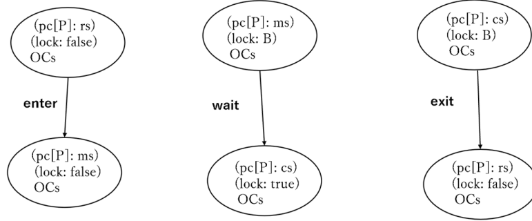
Figure 3.1: Representing the rewriting rules using a figure
