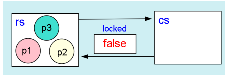
Figure 3.16: Visually representing the state machine using SMGA
