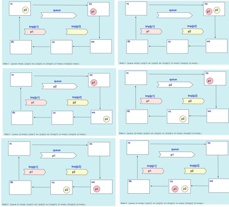
Figure 4.10: Visual representation of various state machines using SMGA(FQlock0)
