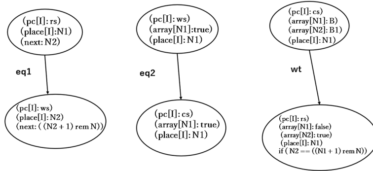
Figure 5.1: Representing rewrite rules using diagrams
