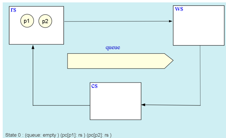
Figure 4.33: Diagram showing the initial conditions using SMGA(Qlock)
