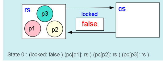
Figure 3.21: Diagram showing the initial conditions using SMGA(TAS)
