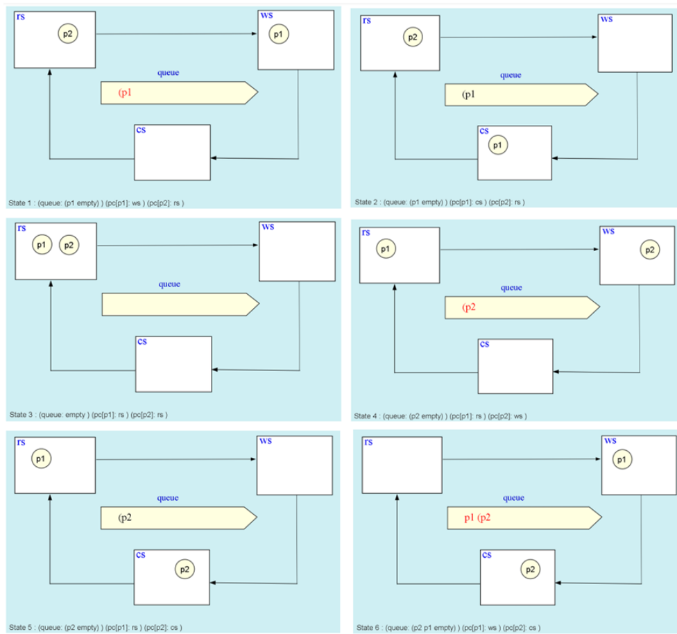
Figure 4.34: Visual representation of various state machines using SMGA (Qlock)
