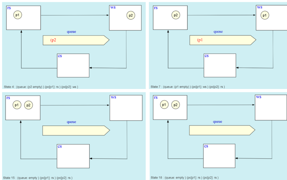
Figure 4.37: When a process exists in rs, it means that the value of the process does not exist in queue.
