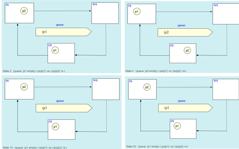
Figure 4.35: Indicates that there can be at most one process in cs.
