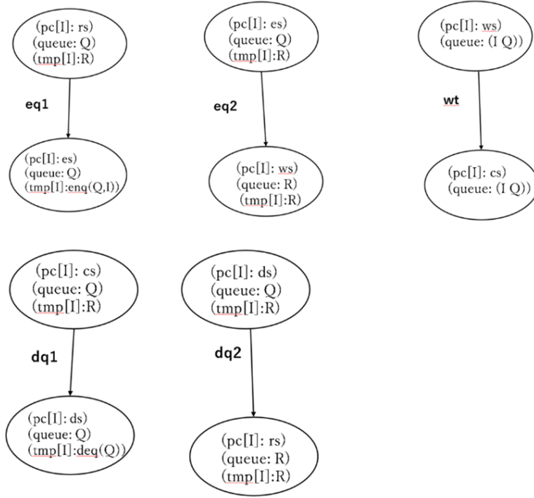
Figure 4.1: Representing the rewriting rules using a figure(FQlock0)
