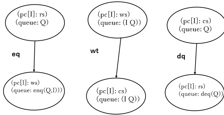
Figure 4.26: Representing the rewriting rules using a figure Qlock
