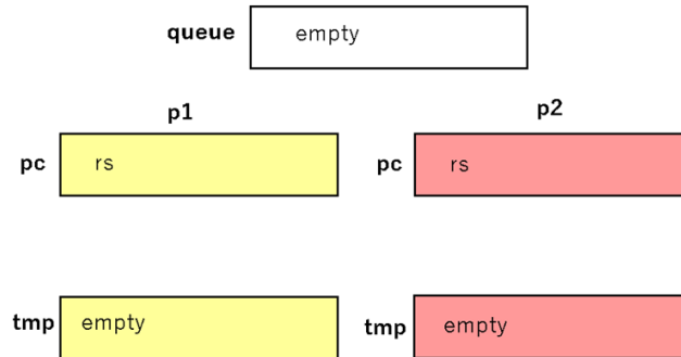
Figure 4.14: Representation of a state machine in a diagram(FQlock1)
