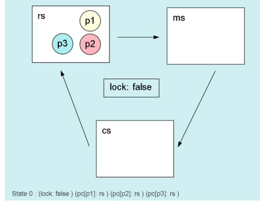
Figure 3.8: Diagram showing the initial conditions using SMGA(FTAS)
