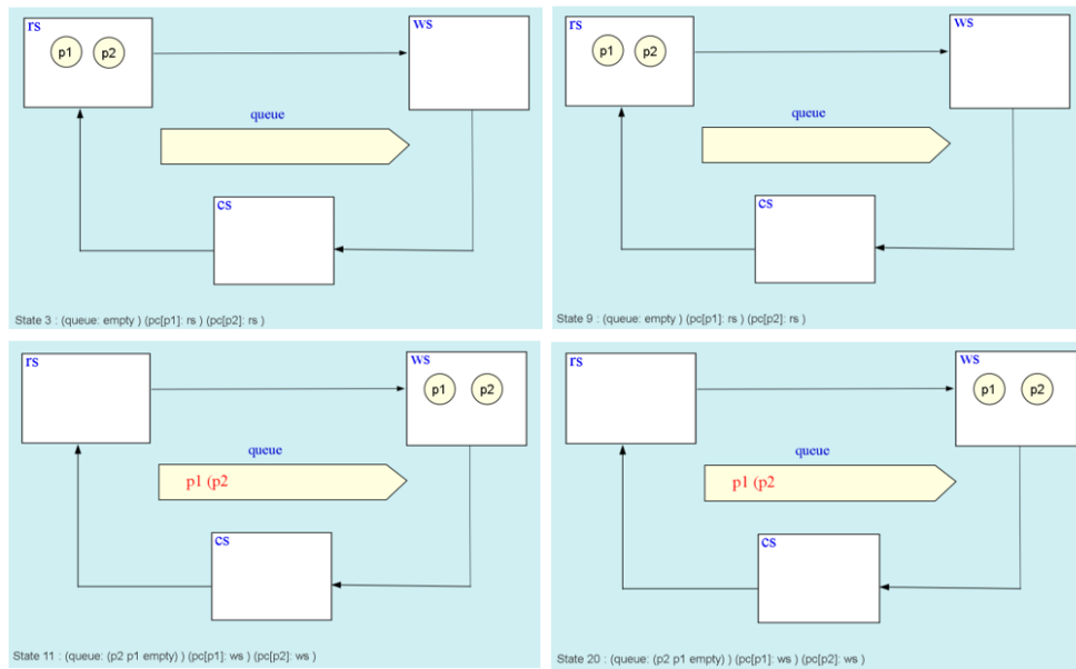
Figure 4.36: It shows that two processes can exist simultaneously in rs and ws.
