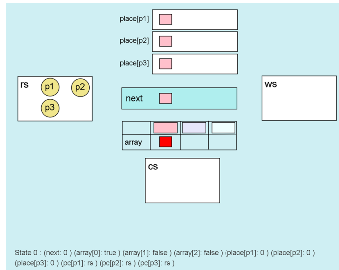
Figure 5.3: Using SMGA to visually represent state machines
