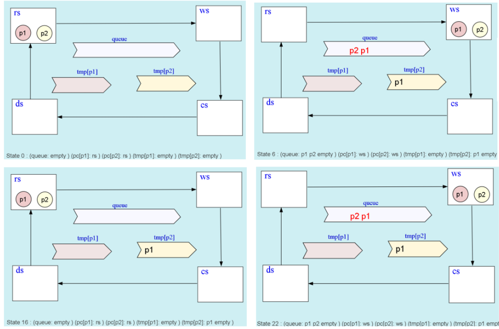
Figure 4.25: It shows that two processes can exist simultaneously in rs and ws.
