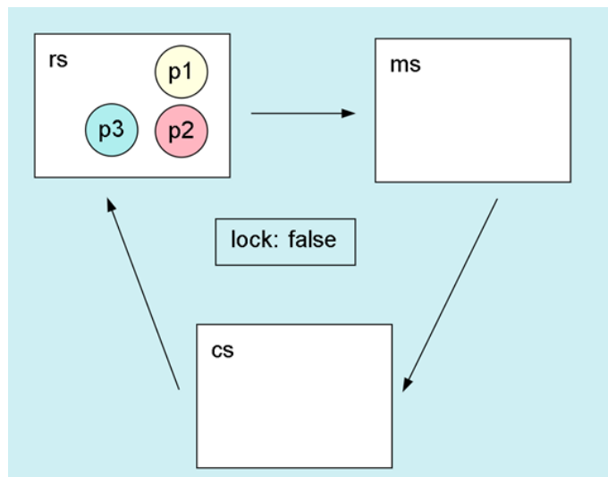
Figure 3.3: Visually representing the state machine using SMGA
