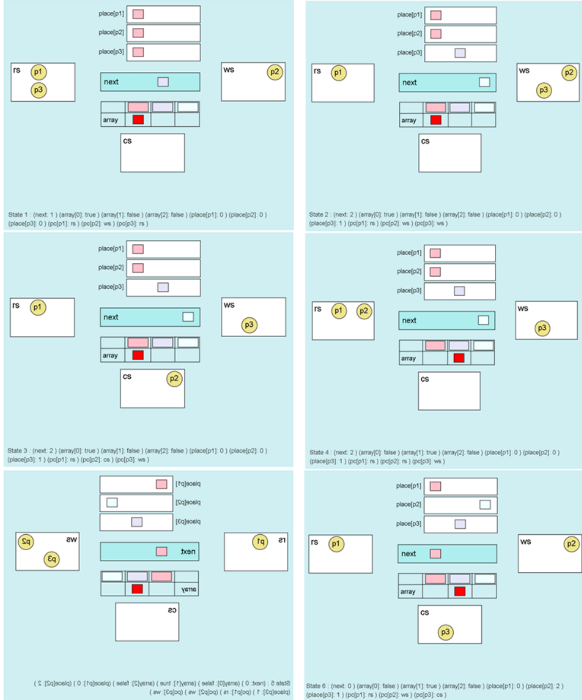
Figure 5.13: Visual representation of various states using SMGA
