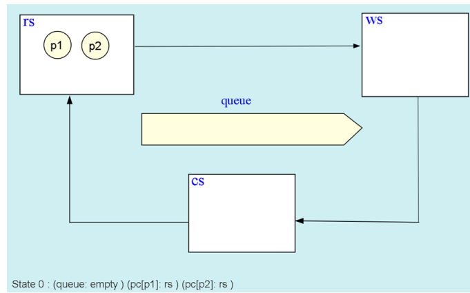
Figure 4.28: Visually representing the state machine using SMGA(Qlock)
