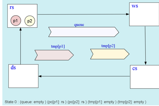
Figure 4.21: Diagram showing the initial conditions using SMGA(FQlock1)
