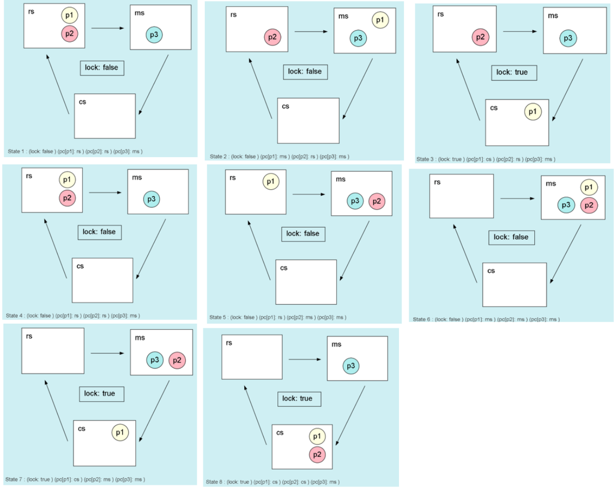
Figure 3.9: Visual representation of various state machines using SMGA
