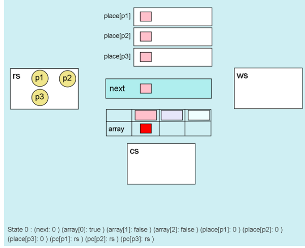
Figure 5.12: Diagram showing the initial conditions using SMGA(Anderson)
