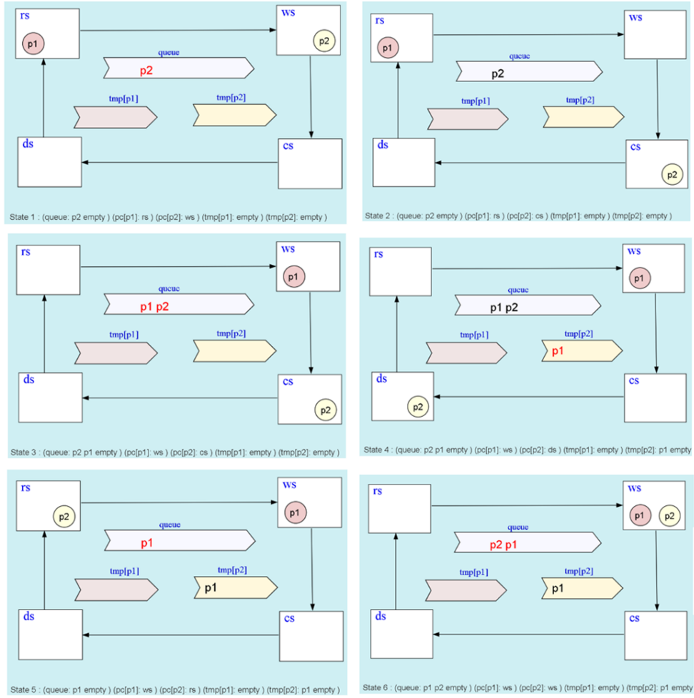
Figure 4.22: Visual representation of various state machines using SMGA(FQlock1)
