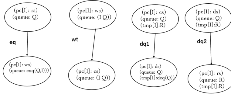
Figure 4.13: Representing the rewriting rules using a figure(FQlock1)
