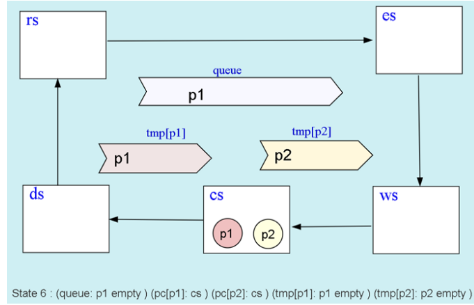
Figure 4.12: Mutual exclusion is not satisfied because two processes can exist simultaneously in cs.
