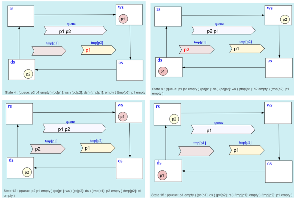
Figure 4.24: It indicates that there is at most one process in ds.
