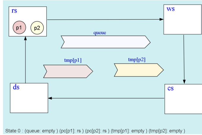
Figure 4.15: Representation of a state machine in a diagram(FQlock1)
