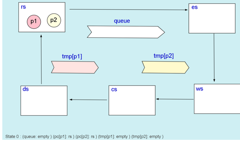
Figure 4.9: Diagram showing the initial conditions using SMGA(FQlock0)
