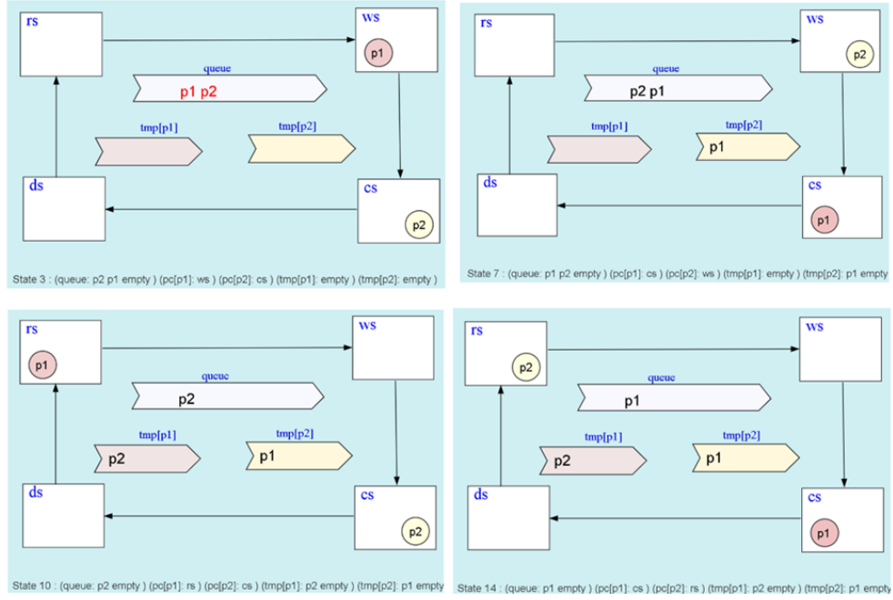
Figure 4.23: It indicates that there is at most one process in cs.
