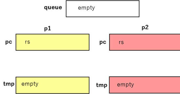
Figure 4.2: Representation of a state machine in a diagram(FQlock0)
