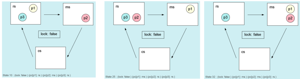
Figure 3.13: Figure showing that if there is no process in cs, the value of “lock” will be false
