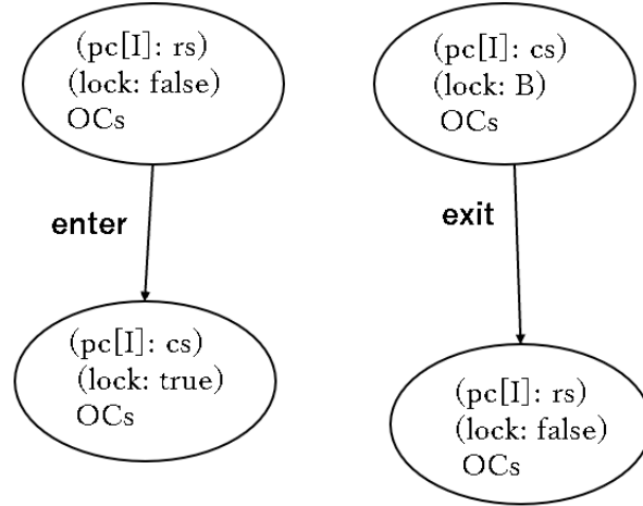
Figure 3.14: Representing the rewriting rules using a figure(TAS)
