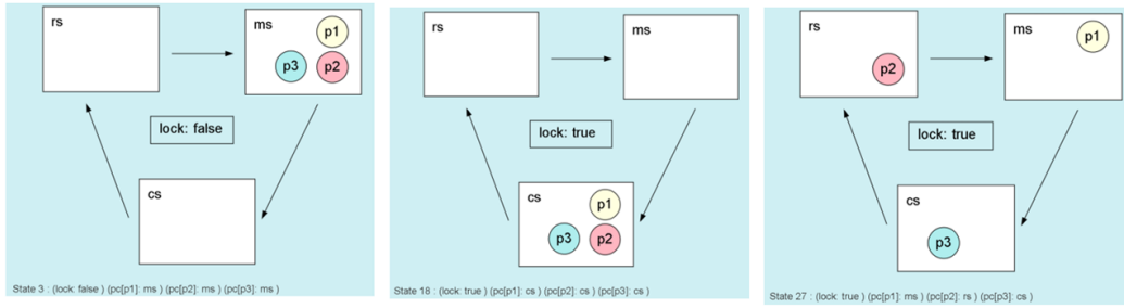
Figure 3.11: Figure showing that there can be up to three processes in each section at the same time.
