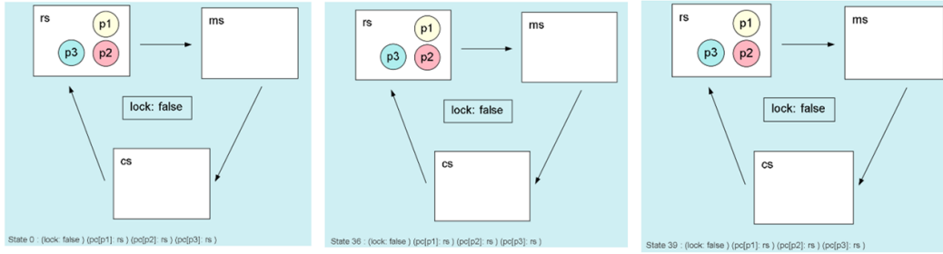
Figure 3.12: Figure showing that the value of “lock” will be false if all processes are present in rs
