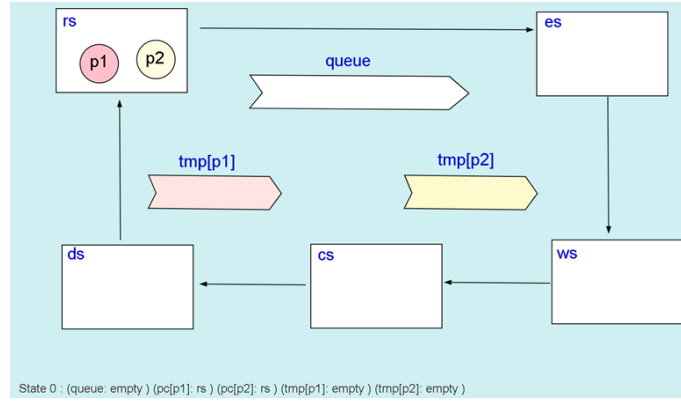
Figure 4.3: Visually representing the state machine using SMGA(FQlock0)
