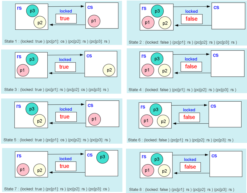
Figure 3.22: Visual representation of various state machines using SMGA(TAS)
