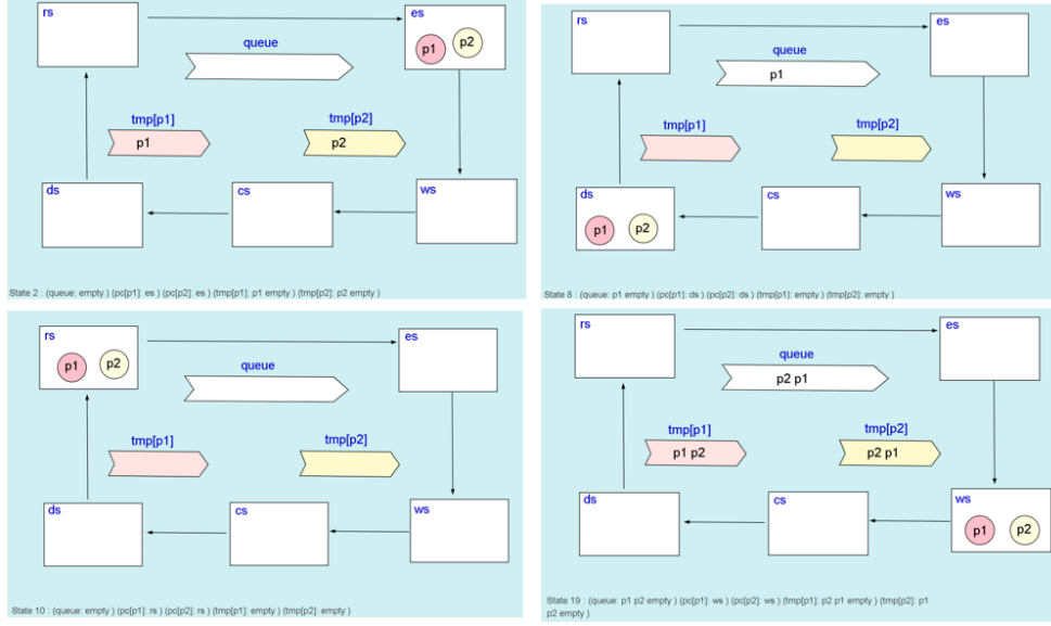
Figure 4.11: There are at most two processes in each section at the same time.
