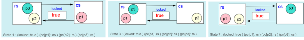
Figure 3.23: Figure showing that there is at most one process in cs.
