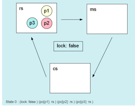
Figure 3.10: The state does not meet the mutual exclusion of the machine
