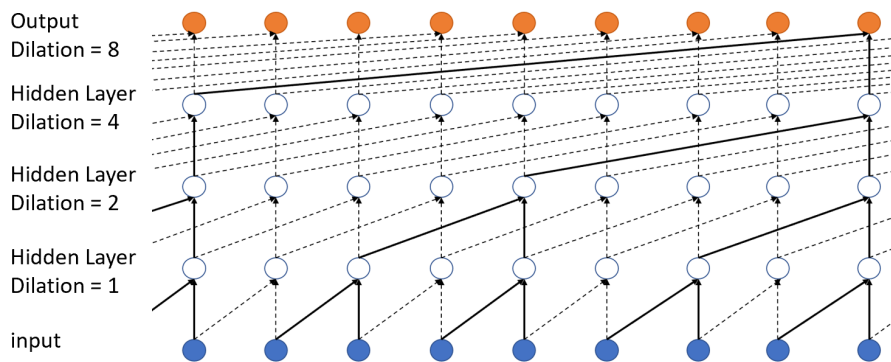
図 4.2: Dilated 1D Causal Convolution の図解
