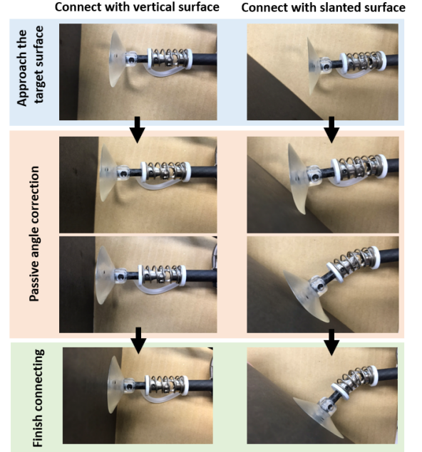
Fig. 2. According to different angles of the surface, the robotic legs work passively, automatically adjusting the vacuum cup's angle when contacting the surface.
