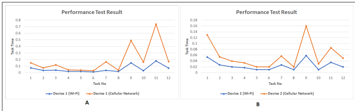
Figure 5.19 The comparison of task time based on the network speed; A. device 1, B device 2 Based on the two-device response time, we draw the following conclusions: First, it is clear that hardware specifications affect AR-GIS performance. The second device has a higher hardware specification. The response system in displaying the map is shorter than the first device. Then panning and the rotating map does not give too much burden to the hardware. The map load consumes more resources when zooming maps. It is because the zoom process changes the map scale. If the map scale changes, the map will load a new tilesets and update the map information. Second, Mapbox stores all maps in cloud storage media. Therefore, internet speed affects map loading time. It is getting longer on poor internet connection. As we see in Figure 5.12, there are differences in task times on the same device but using different internet speeds. Finally, the tasks that require the longest response time are tasks 1, 2, 7, 9, and 11. These five tasks are tasks that require the system to load tilesets from the cloud. These two conclusions are in line with other studies[50], [82], [92], [101]. Other study result state that hardware capabilities and internet networks have a significant influence on system performance. However, based on the performance testing result in table 5.4, the maximum response time on the system is 0.180 seconds. This value is still categorized as a Short Response Time so that it does not affect the user's activity on the application[102].
