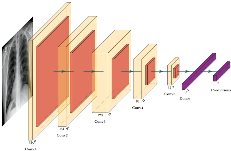
Figure 4.1: Covid Model Archtutre.
