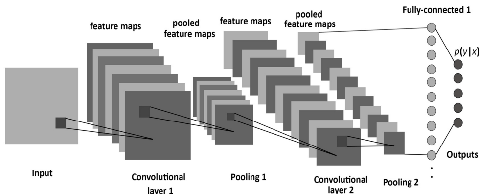
Figure 3.4: CNN structure[1]
