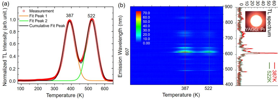
Figure 5. a) TL glow curve of the YAGG: \text{Pr}^{3+} transparent ceramic with a heating rate of 10 \text{ K min}^{-1} . The sample was irradiated by UV light (250 to 380 nm) from a mercury lamp for 5 min. b) Wavelength–temperature ( \lambda - T ) 2D TL contour mapping of the YAGG: \text{Pr}^{3+} transparent ceramic. The right projection shows the TL emission spectrum at 387 and 522 K.
