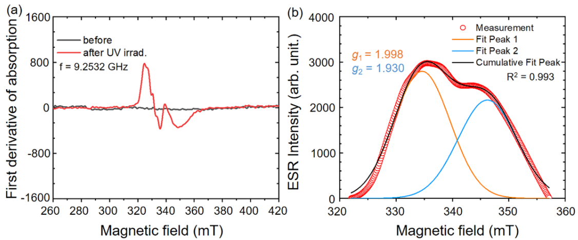
Figure 6. a) ESR spectra of YAGG: Pr 3+ transparent ceramic before (black) and after 5 min UV irradiation (red) in the X band at room temperature. b) Decomposition of the ESR line after UV irradiation into two Gaussian components demonstrating anisotropy of the g factor.
