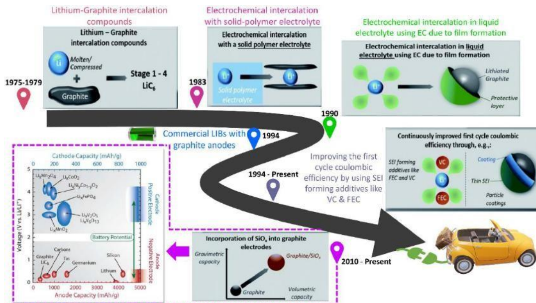
Figure 9 LIB technology - from its origin to the recent advancements
