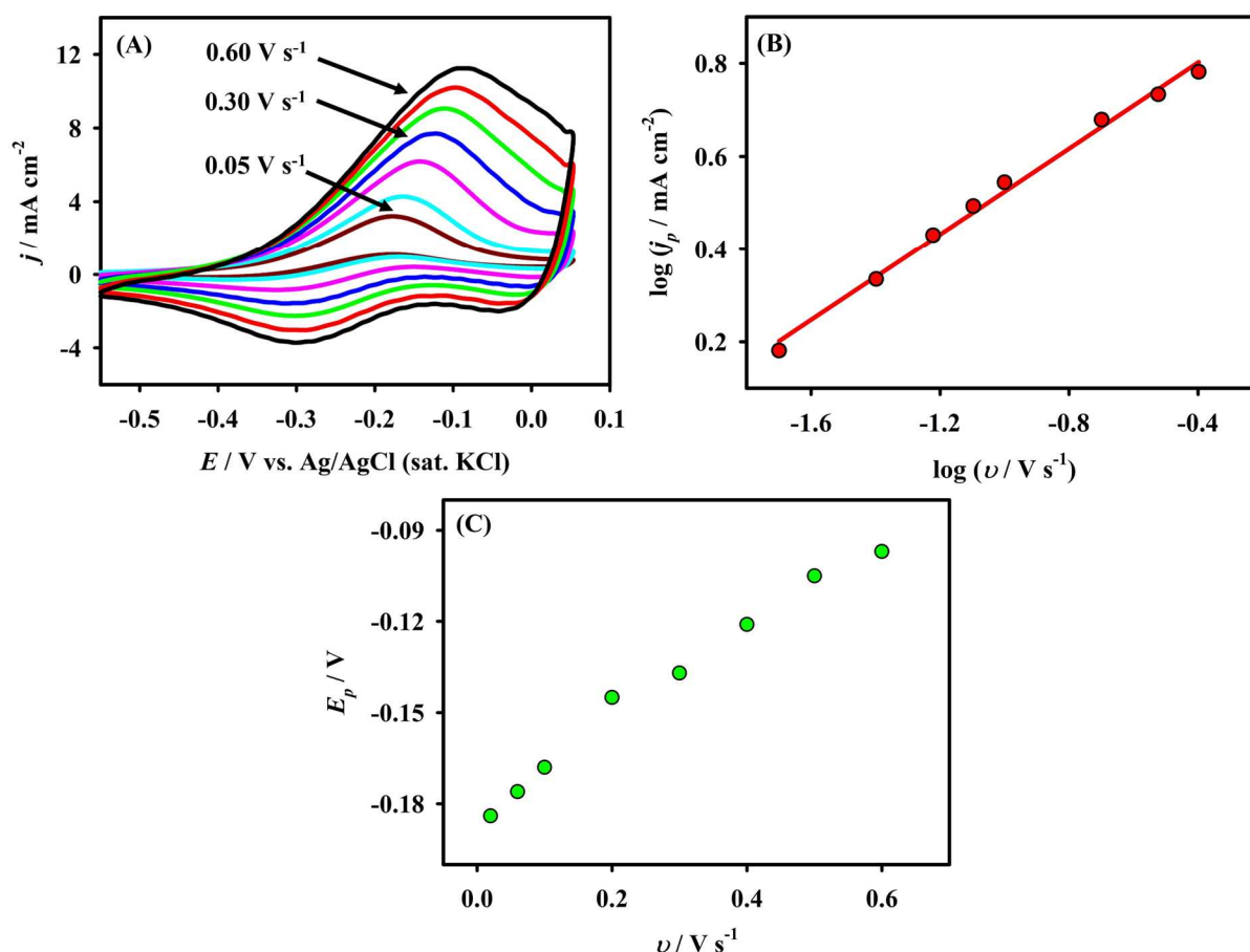
Figure 8. (A) Scan rate dependent cyclic voltammograms of IrO x -Pt in 1.0 M N 2 -saturated NaOH solution having 0.25 M ethanol, (B) Logarithmic relationship between anodic peak current densities and scan rates, (C) Variation of anodic peak potentials with respect to scan rates.
