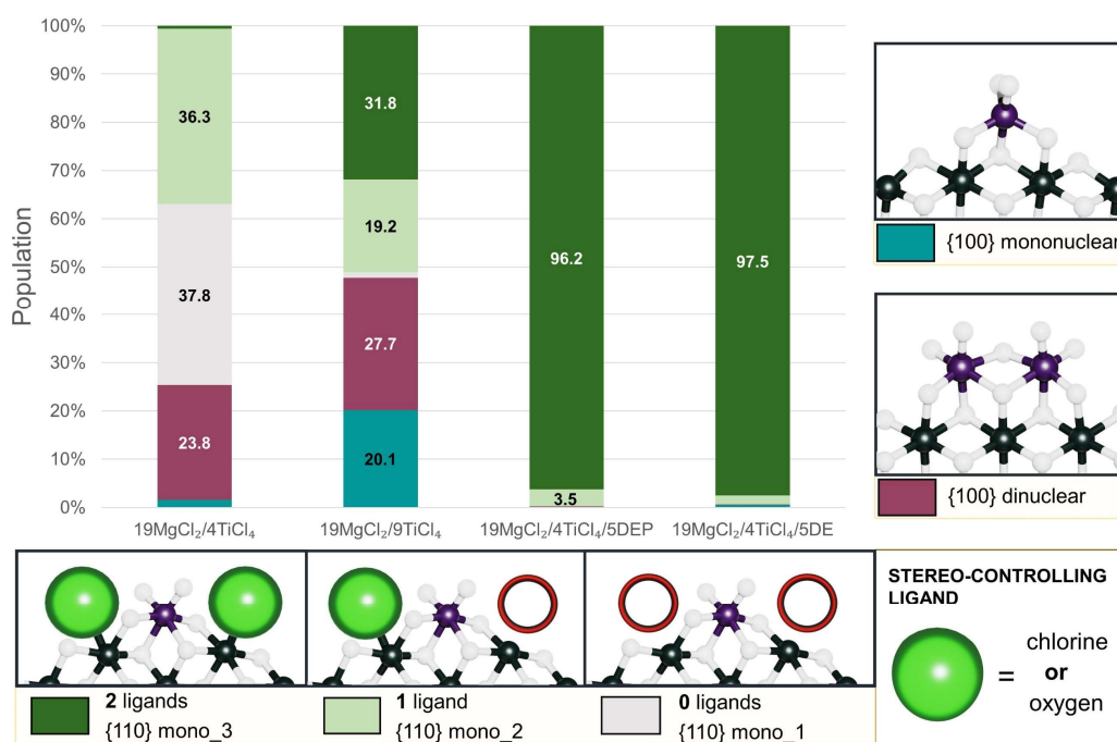
Figure 2: Population of \text{TiCl}_4 species, classified according to the adsorption mode and, in the case of \{110\} mononuclear, presence of stereo-controlling ligands.
