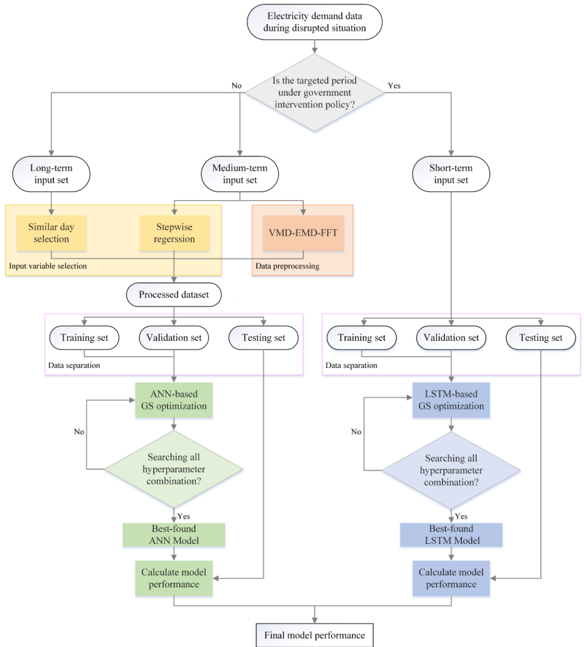
Figure 1 Overall procedure of the proposed models.
