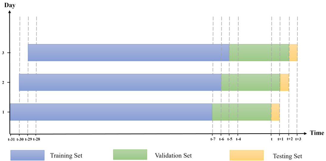
Figure 4 Walk-forward testing technique for the rolling dataset.
