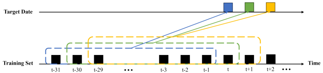
Figure 3 One-day-ahead forecasting technique.
