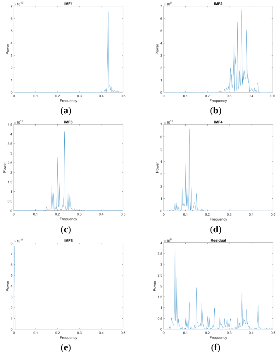
Figure 13 Identification of seasonality and trends using FFT analysis for all IMFs and residuals: (a) IMF1; (b) IMF2; (c) IMF3; (d) IMF4; (e) IMF5; (f) Residual.
