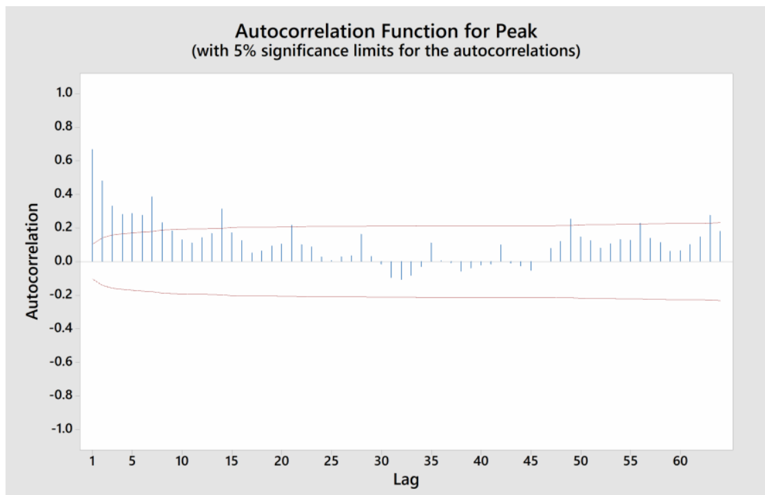
Figure 6 Analysis of autocorrelation in electricity peak demand amid the COVID-19 pandemic.
