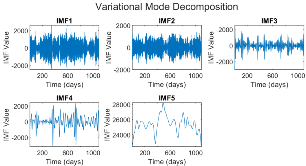
Figure 11 Decomposition results of VMD, breaking down the electricity peak demand from 2018 to 2020 into IMFs (IMF1 to IMF5).
