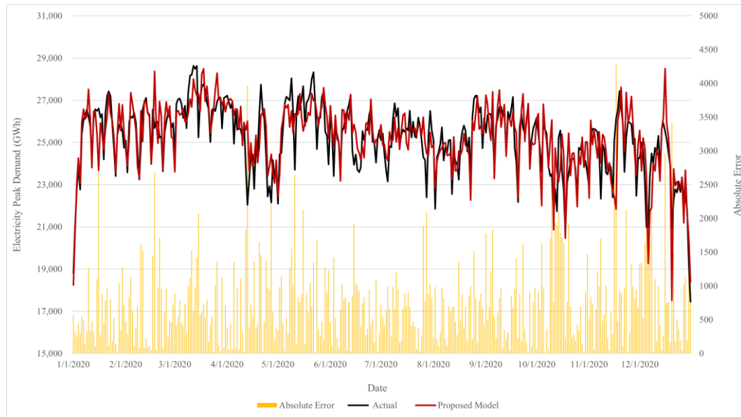
Figure 14 Daily forecasting errors of proposed procedure on test dataset.
