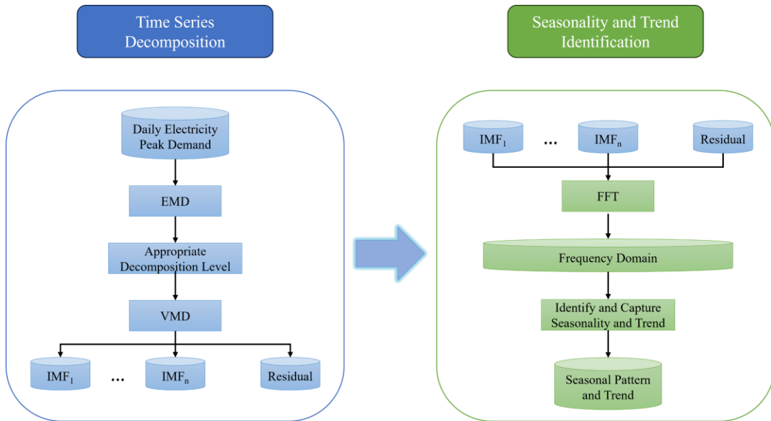
Figure 2 Flowchart of data decomposition and seasonality identification process.
