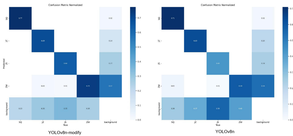
Figure 5-3: Confusion matrix
