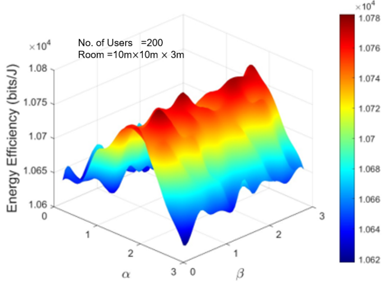
Figure 4.16: Energy efficiency analysis in multi-user VLC
