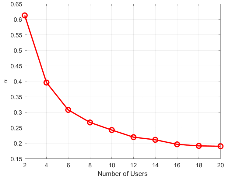
Figure 4.6: Performance of \alpha versus no. of users for ADO-OFDM NOMA
