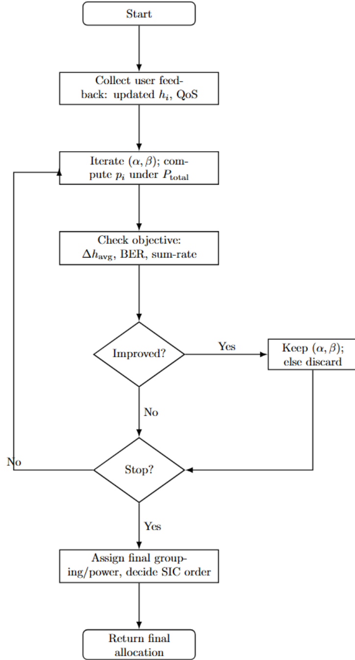
Figure 3.13: Flowchart of power allocation and four-user pairing for MCGAD NOMA
