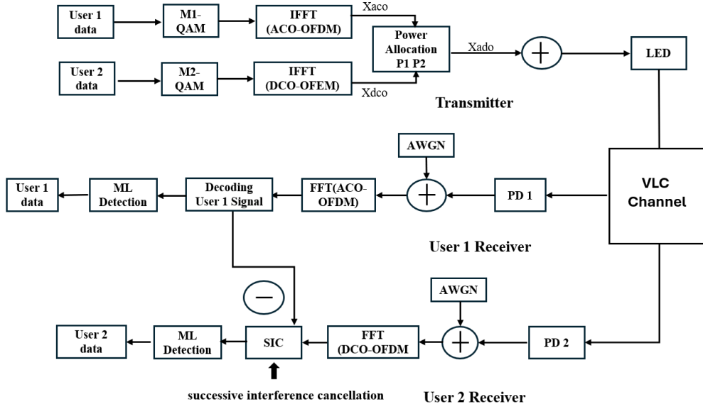
Figure 3.2: Two-user ADO-OFDM NOMA for VLC
