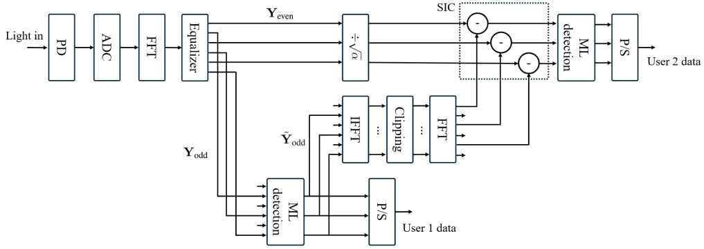
Figure 3.4: Proposed ADO-OFDM NOMA receiver
