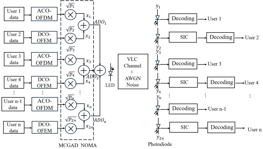
Figure 3.6: Proposed MCGAD NOMA for multi-user VLC
