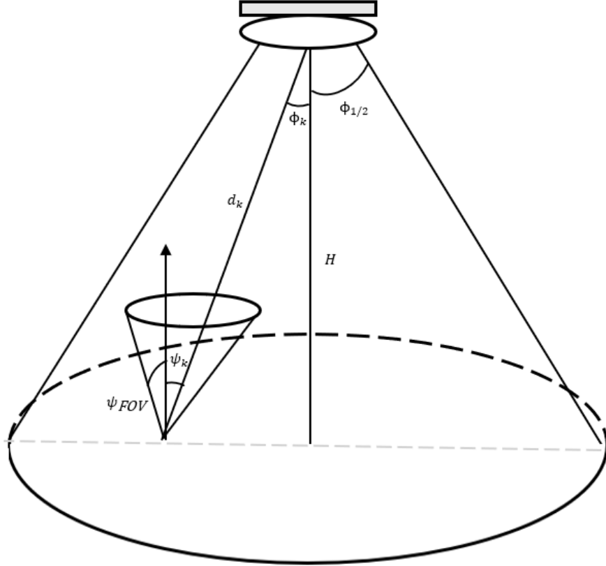
Figure 2.1: Illustration of an indoor VLC system
