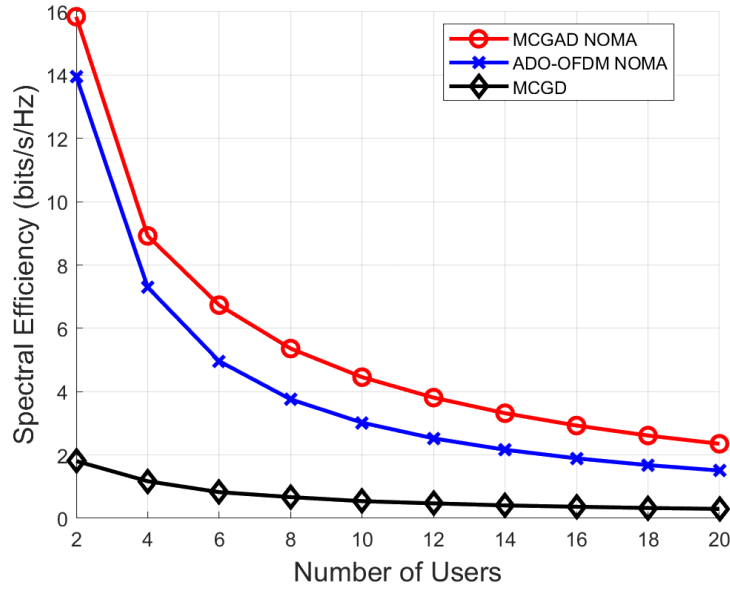
Figure 4.13: Performance of spectral efficiency for multi-user VLC scenario
