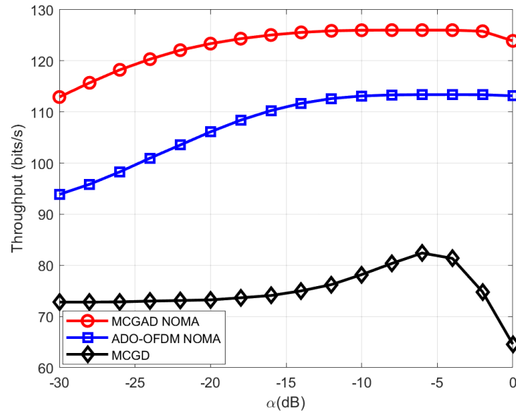
Figure 4.11: Performance of throughput versus \alpha for various schemes in four-user VLC scenario
