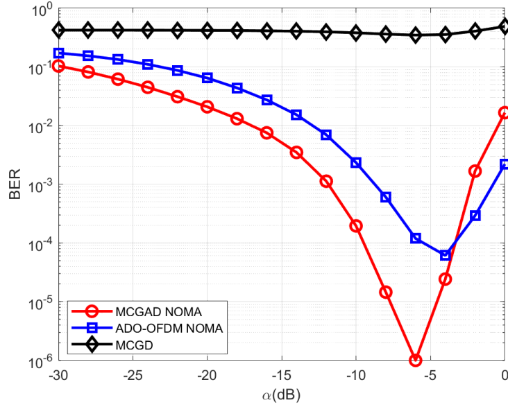
Figure 4.9: Performance of BER versus \alpha for various schemes in four-user VLC scenario
