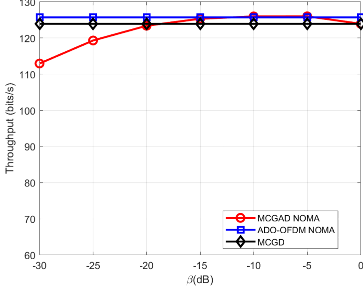
Figure 4.12: Performance of throughput versus \beta for various schemes in four-user scenario
