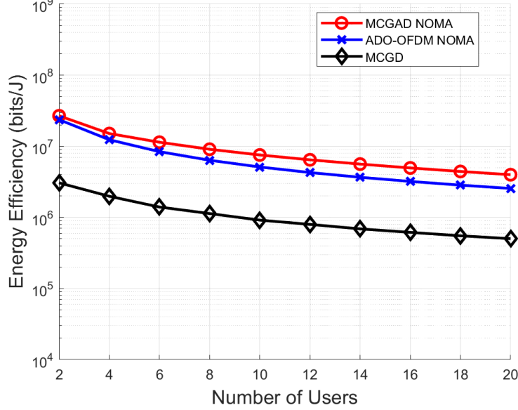
Figure 4.14: Performance of energy efficiency for multi-user VLC scenario
