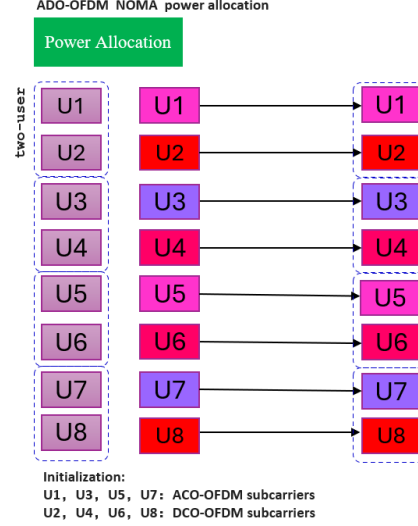
Figure 3.8: Proposed grouping scheme of ADO-OFDM NOMA for multi-user VLC
