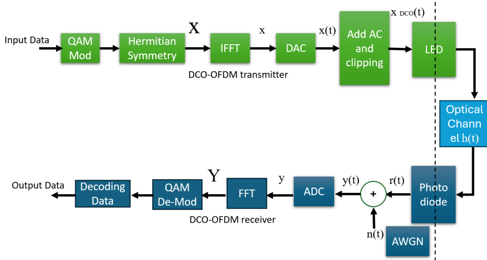
Figure 2.7: Illustration of DCO-OFDM
