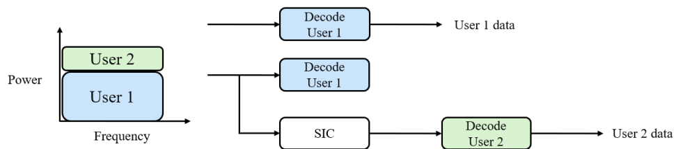
Figure 2.10: Conceptual diagram of NOMA SIC
