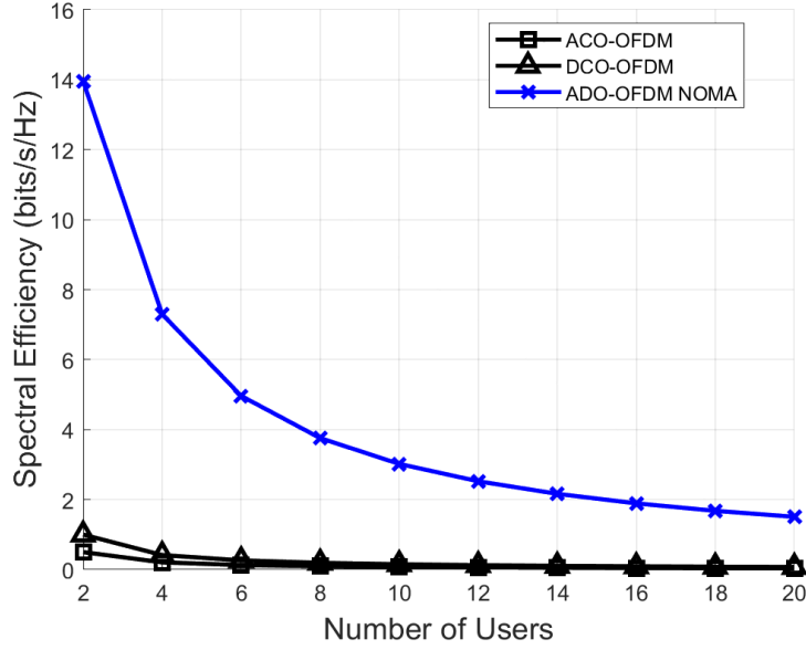
Figure 4.4: Performance of spectral efficiency versus no. of users
