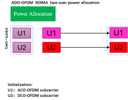
Figure 3.7: Proposed grouping scheme of ADO-OFDM NOMA for two-user VLC
