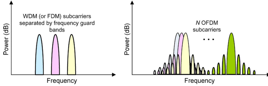
Figure 2.4: Illustration of OFDM subcarrier orthogonality [4].
