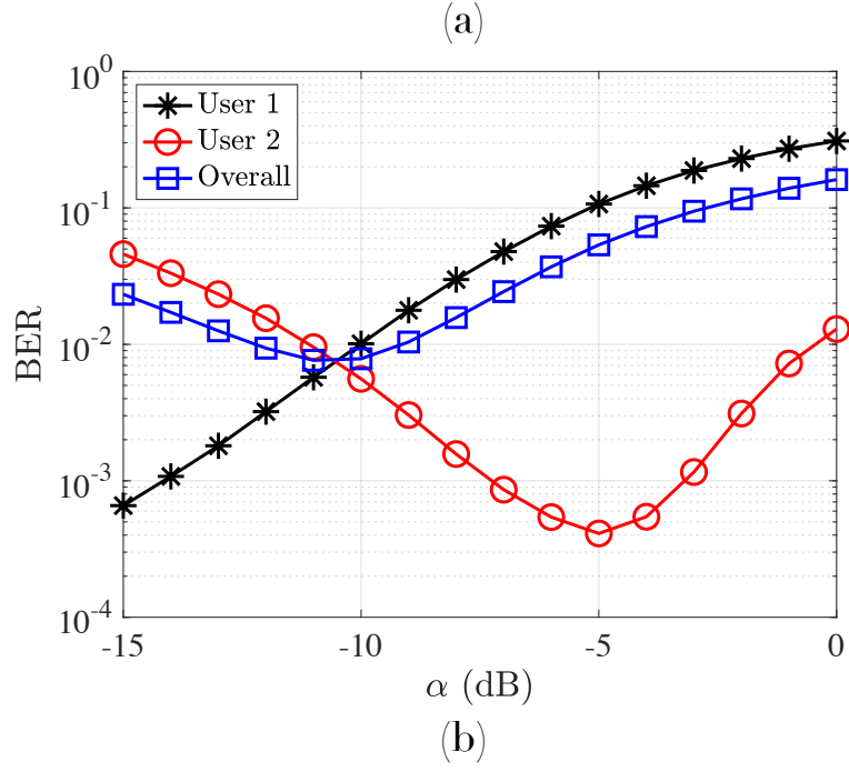
Figure 4.2: BER vs. \alpha when two users are closely spaced with a 10 dB DC bias.
