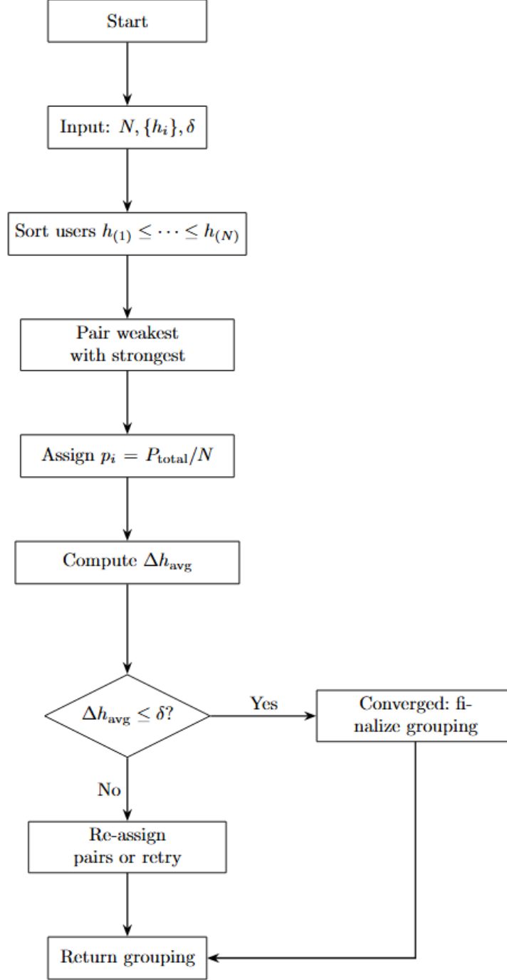
Figure 3.12: Flowchart of initialization & detection algorithm for MCGAD NOMA
