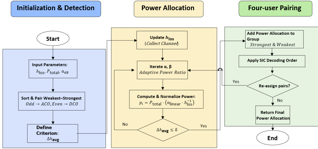
Figure 3.10: Flowchart of power allocation and user grouping for MCGAD NOMA
