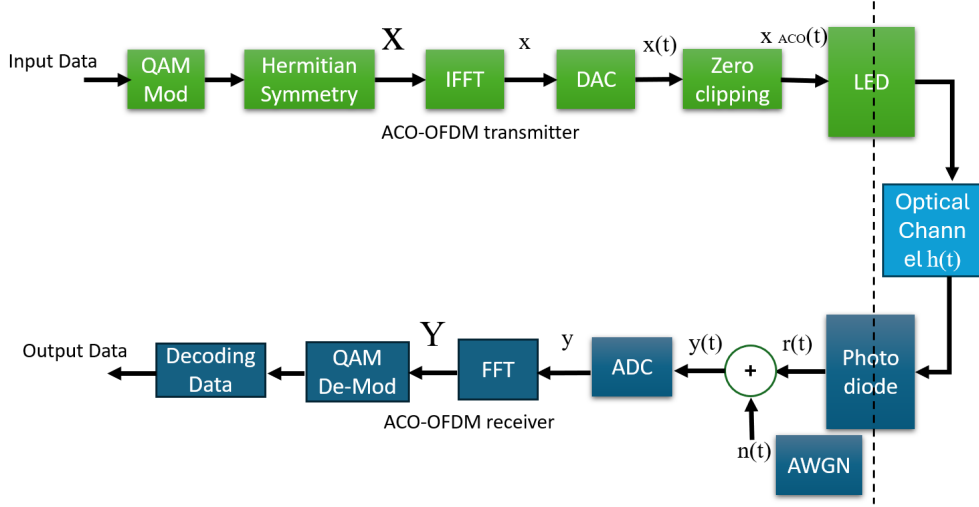
Figure 2.6: Illustration of ACO-OFDM
