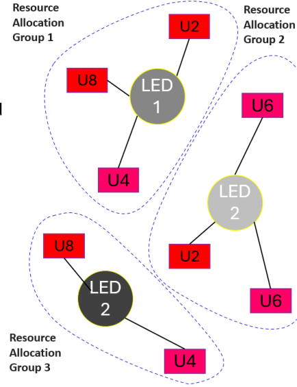
Figure 2.13: Grouping scheme based on k-means algorithm [7].
