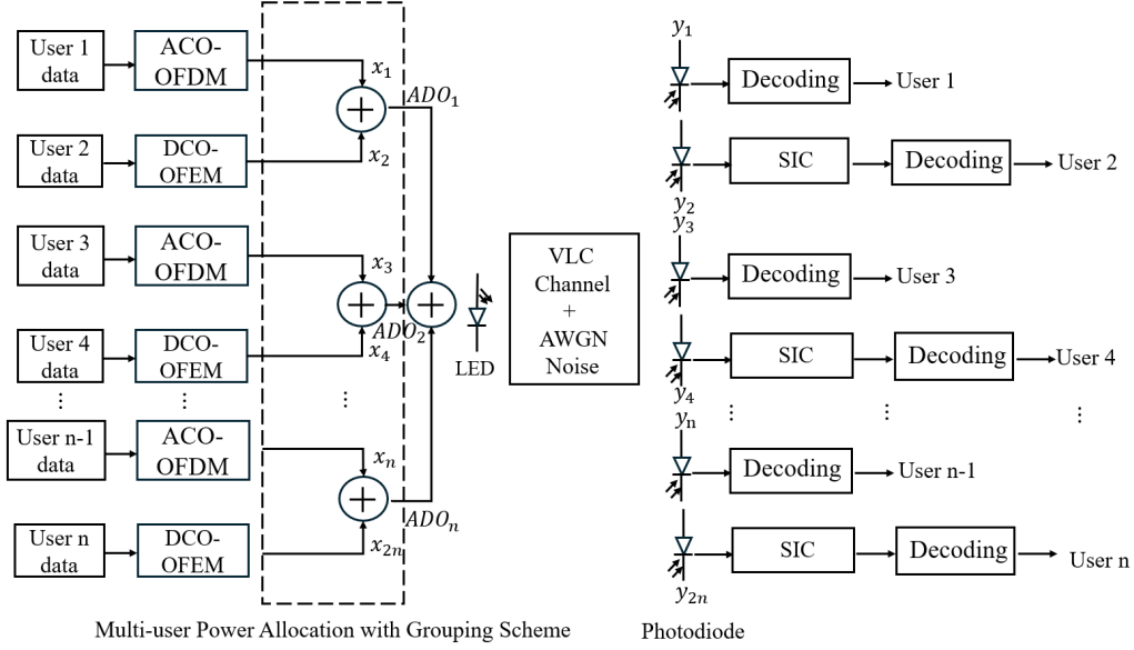
Figure 3.5: Proposed ADO-OFDM NOMA for multi-user VLC
