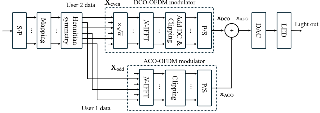
Figure 3.3: Proposed ADO-OFDM NOMA transmitter
