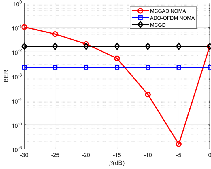
Figure 4.10: Performance of BER versus \beta for various schemes in four-user VLC scenario
