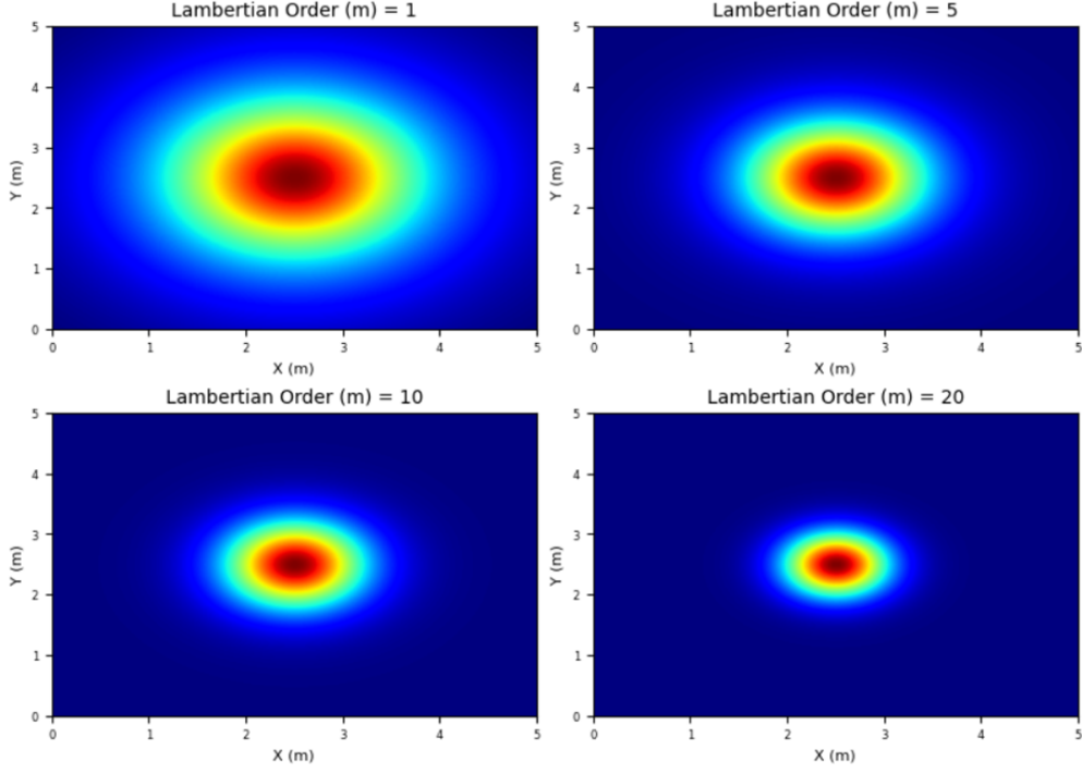
Figure 2.3: Lambertian radiation pattern
