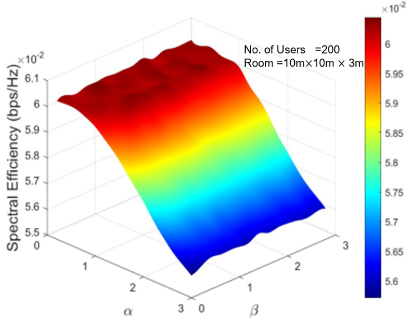
Figure 4.15: Spectral efficiency analysis in multi-user VLC
