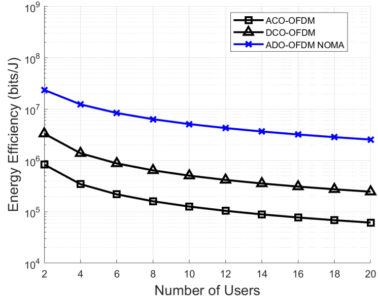
Figure 4.5: Performance of energy efficiency versus no. of users
