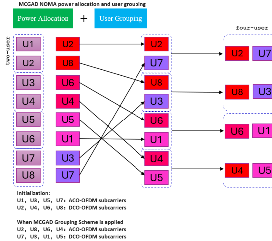
Figure 3.9: Proposed grouping scheme for MCGAD NOMA for multi-user VLC
