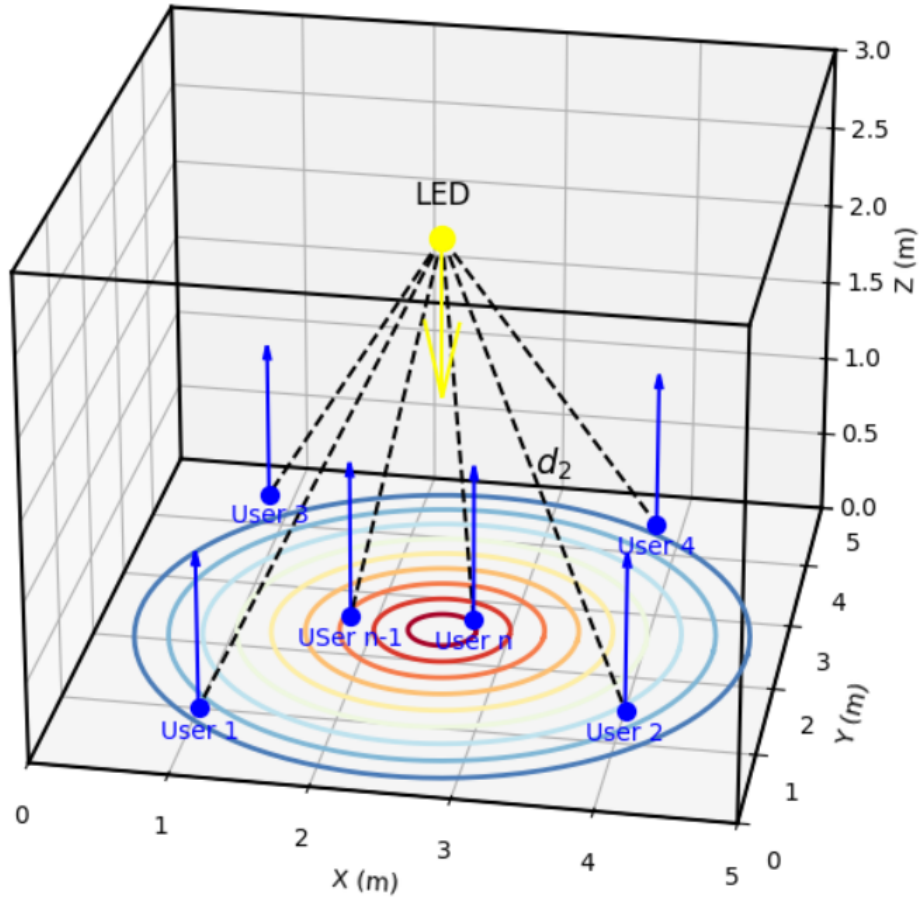
Figure 4.1: Illustration of simulation environment for ADO-OFDM NOMA and MCGAD NOMA in Multi-user VLC.
