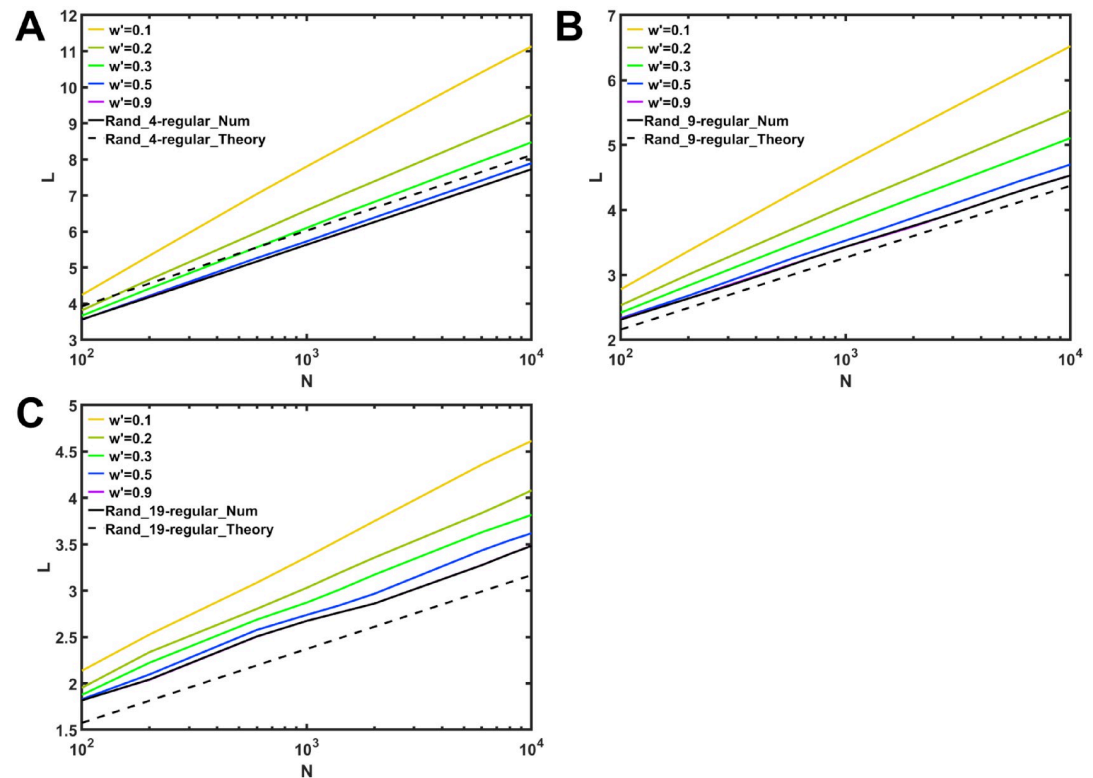
Fig 6. Disparities of average path length L between the values for rewired modular networks and theoretical value. Rewired networks with (A) d = 4 , N_m = 20 , (B) d = 9 , N_m = 20 , and (C) d = 19 , N_m = 20 . Color lines represent a rewiring rate w' on anti-modularization. Black solid and dashed lines indicate numerical and theoretical values for random d -regular graphs without modular structures.
