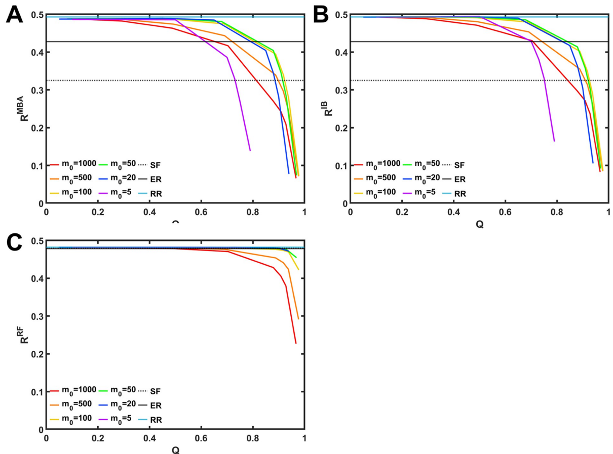
Fig 3. Relation between modularity Q and robustness index R against three types of attacks. (A) R_{MBA} against MB, (B) R_{IB} against IB, and (C) R_{RF} against RF. Color lines represent the results for the number m_0 of modules. Black solid, dotted, and cyan lines represent the robustness after these attacks in non-modular ER, SF networks and random d -regular graphs.
