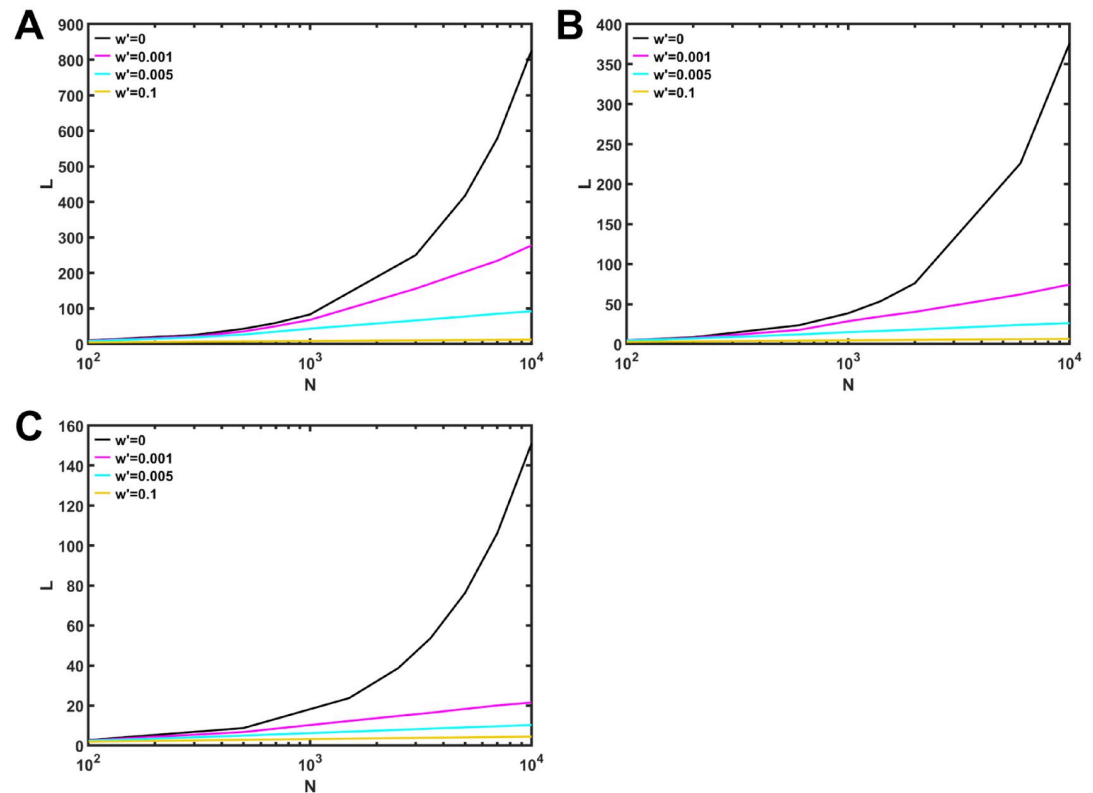
Fig 5. Average path length L in rewired networks for varying the network size N . Rewired networks with (A) d = 4 , N_m = 10 , (B) d = 9 , N_m = 20 , and (C) d = 19 , N_m = 50 . Color lines represent a rewiring rate w' on anti-modularization.
