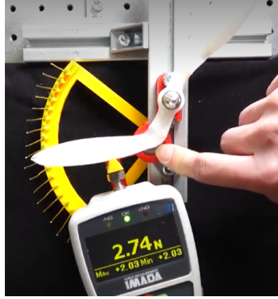
Figure 4.9: The experiment setup for stiffness of joint k .
