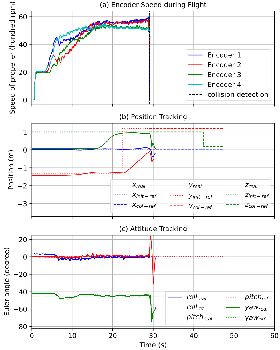
Figure 4.29: Experimental results of collision detection and response for a quadrotor equipped with rigid propellers while flying toward the target point.
