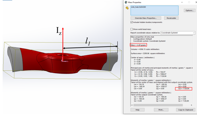
Figure 4.7: Inertia moment J_1 and haft-length l_1 of link hub (SolidWorks)
