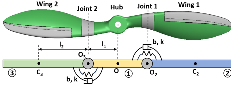
Figure 4.6: Modeling of deformable propeller
