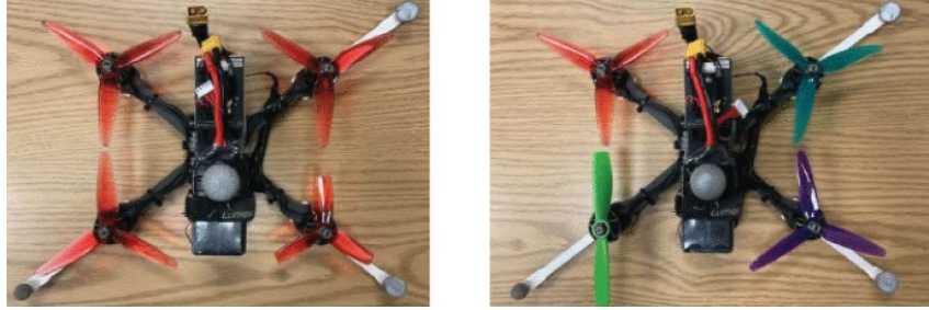
(c) Quadrotors with chipped propeller and mixed propellers.
