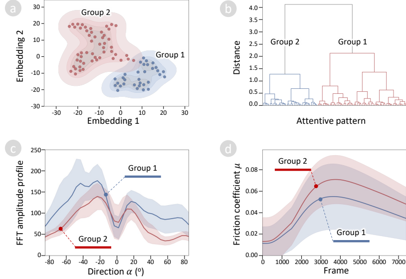
Figure 4.11: Clustering attentive organizational patterns in wet rubber-surface contact. (a) t-SNE embedding of angular coherence profiles across all experiments. (b) Hierarchical clustering dendrogram computed from DTW distances. (c) Representative angular coherence profiles of the two identified groups. (d) Temporal evolutions of friction coefficient \mu for experiments in each group.
