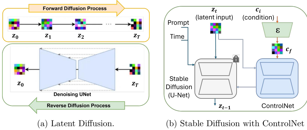
Figure 2.3: (a) Latent Diffusion: the model learns to denoise latent variables from z_T to z_0 through a U-Net. (b) Stable Diffusion with ControlNet: encodes condition input c_i into guidance features to modulate the denoising of latent input z_t .
