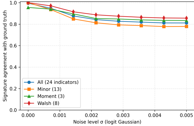
Figure 4.4: Signature agreement under logit–Gaussian noise. Curves correspond to minor, moment, Walsh, and full 24-dimensional signatures and clearly indicate a robust regime in which MIC signatures tolerate noise.
