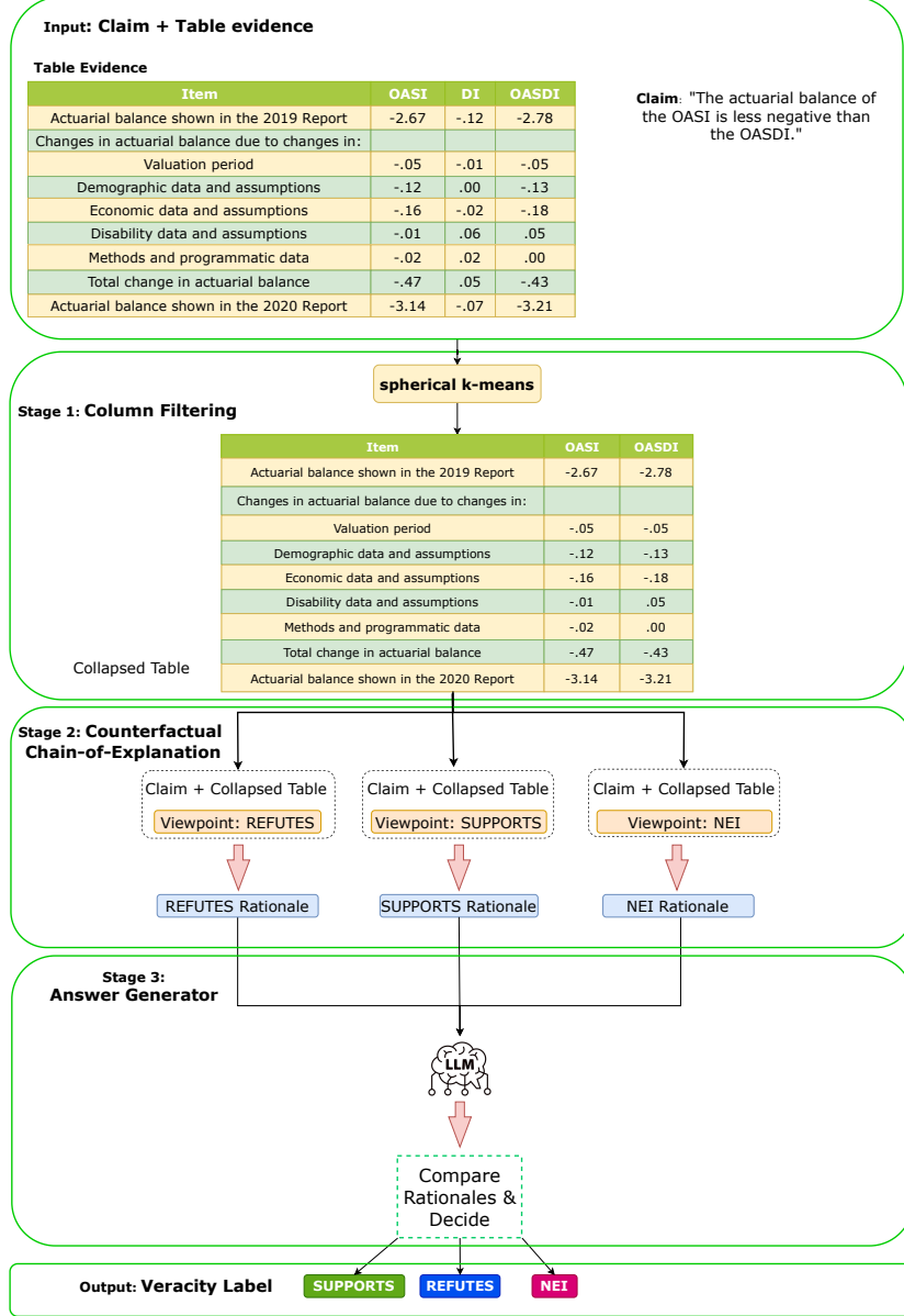
Figure 3.2: An overall framework of UCRET, which contains three main modules: (i) Column Filtering, which selects columns that are relevant to the query to make a collapsed evidence table; (ii) Counterfactual Chain-of-Explanation, which offers detailed reasoning, evaluating how effectively each explanation aligns with the claim by highlighting both its strengths and limitations; and (iii) Answer Generator, which produces the final decision of the claim.
