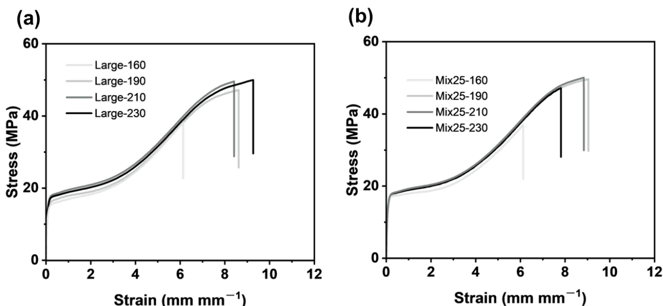
Figure 3.4. Stress-strain curves of pristine UHMWPE films prepared at different temperature: a) Large- \gamma , and b) Mix25- \gamma , where \gamma represents the compression temperature.
