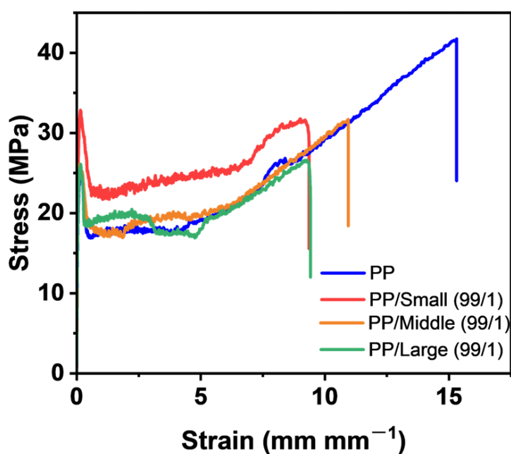
Figure 4.4. Stress-strain curves of PP and PP/UHMWPE with different UHMWPE particle sizes. (Blue) PP, (red) PP/Small (99/1), (orange) PP/Middle (99/1), and (green) PP/Large (99/1).
