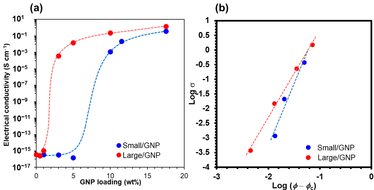
Figure 2.7. Electrical conductivity of nanocomposites: a) Relationship between electrical conductivity and GNP loadings, and b) plots of \log \sigma versus \log (\phi - \phi_c) above the percolation threshold.
