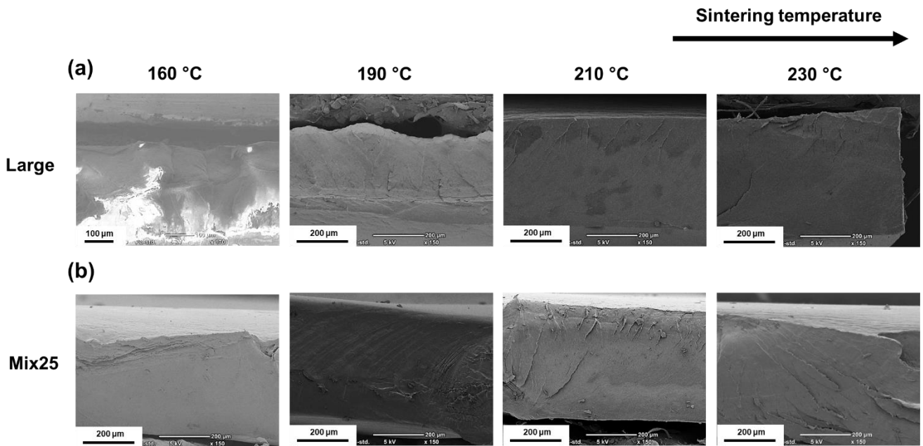
Figure 3.3. SEM images of cryo-fractured surface of pristine films: a) Large, and b) Mix25 prepared at different temperatures. The much smoother fractured surface observed in Mix25 especially at a low sintering temperature demonstrates that incorporating smaller UHMWPE particles enhances particle packing and sintering behavior in the matrix.
