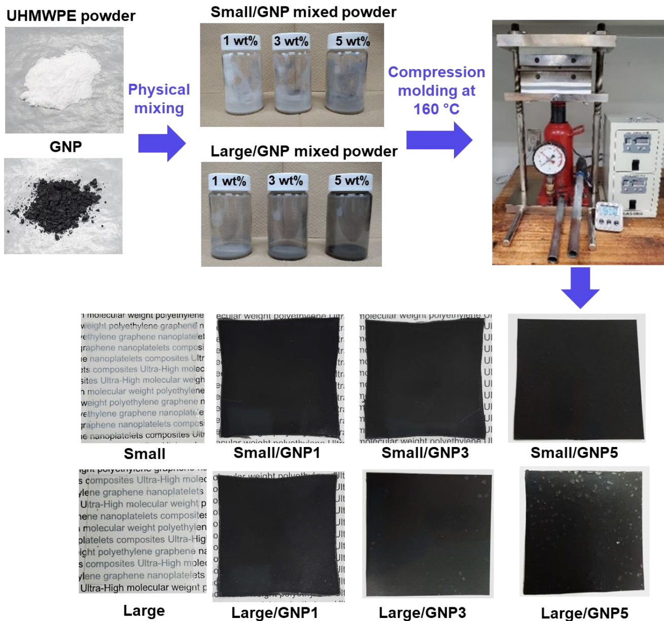
Figure 2.2. Film preparation process and appearance of samples before and after compression molding.
