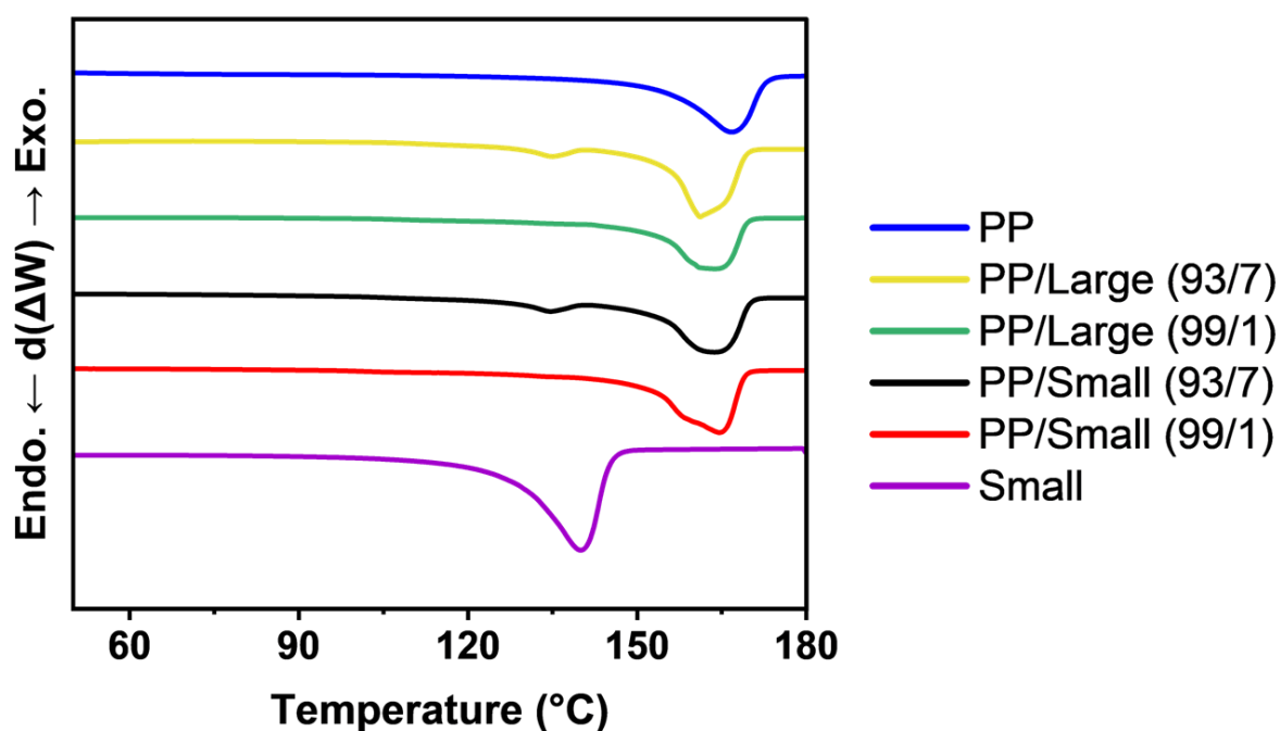
Figure 4.2. DSC curves of first heating cycle for PP, PP/UHMWPE, and Small at a heating rate of 10 °C min -1 .
