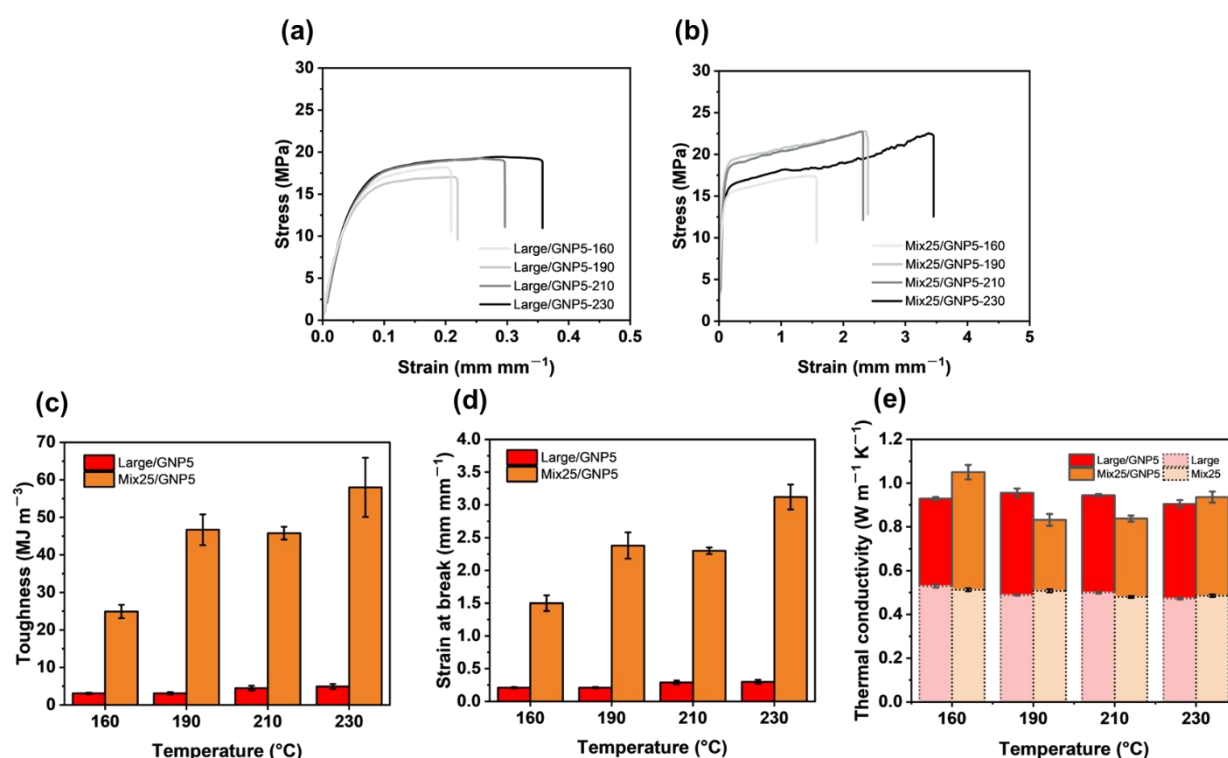
Figure 3.8. Stress-strain curves of obtained UHMWPE/GNP nanocomposites with Large and Mix25 matrices: a) Large/GNP5-y, b) Mix25/GNP5-y, where y represents sintering temperature. (c) Toughness, (d) strain at break, and (e) thermal conductivity of Large/GNP and Mix25/GNP at different sintering temperature.
