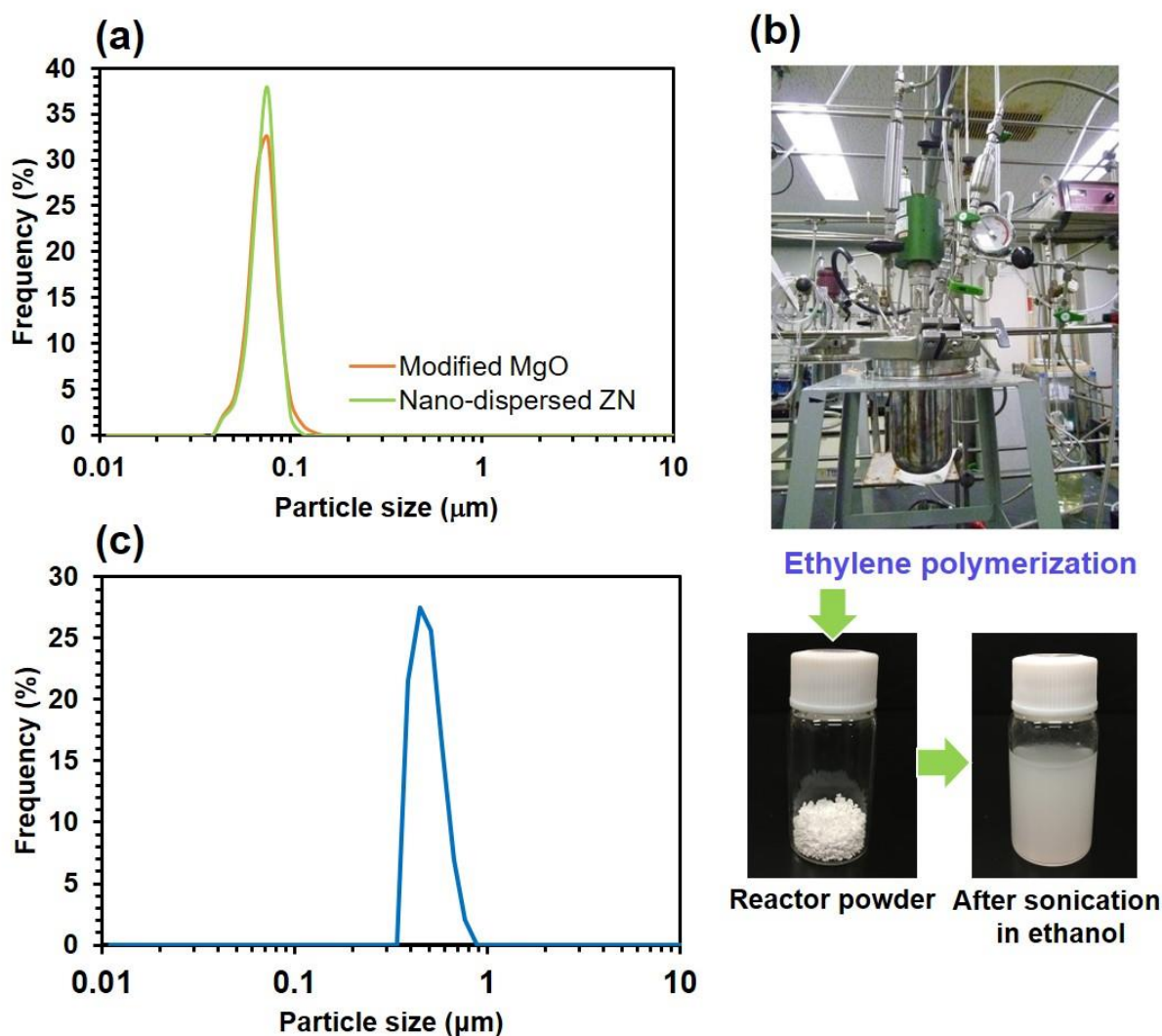
Figure 2.1. A nano-dispersed catalyst and obtained polymers: a) Number-based particle size distribution of organically modified MgO and the resultant catalyst, b) appearance of as-obtained reactor powder and after redispersion by sonication in ethanol, and c) number-based particle size distribution of polymer powder after redispersion.
