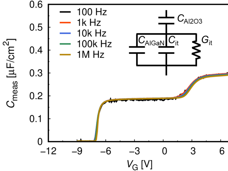
FIG. 5: f -dependent C - V characteristics of the metal/ \text{Al}_2\text{O}_3 / \text{AlGaIn} / \text{GaIn} MIS device with d_{\text{Al}_2\text{O}_3} = 22 nm. Inset: the equivalent circuit.
