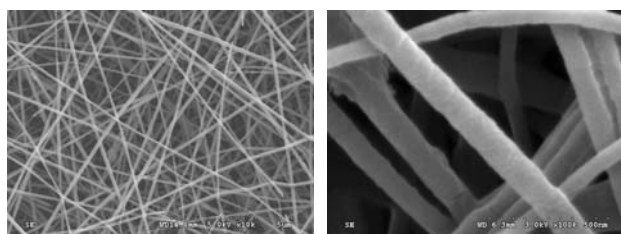
Figure 10 SEM images of electro-spun nanofiber from polypseudorotaxanes between PEO and \alpha -cyclodextrin.
