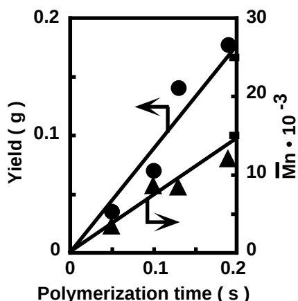
Fig.1. Relationship between yield (●) and \bar{M}_n (▲) of poly(1,5-hexadiene) against polymerization time. Conditions : [1,5-hexadiene] = 1.0 mol/L, [TEA] = 0.07 mol/L, Al/Ti molar ratio = 30
