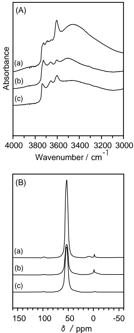
Fig.1: FT-IR and ^{27}\text{Al} MAS NMR spectra of HZSM-5 zeolites of (a) parent, (b) after thermal dealumination at 600 for 48h and (c) after treatment of (b) with 2M HCl at 100 for 120h
