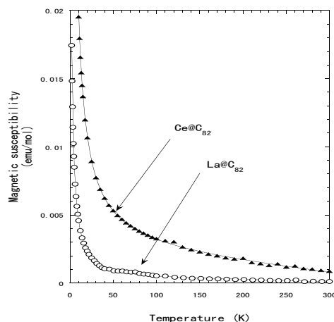
Fig. 2 Temperature dependence of magnetic susceptibility of \text{Ce/La}@\text{C}_{82}
